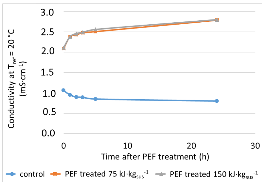
Fig. 1. Conductivity of S. almeriensis suspension after PEF treatment. Biomass obtained from annular PBR and concentrated to 97 g·kg SUS -1 . PEF treated at an energy input of 75 kJ·kg SUS -1
