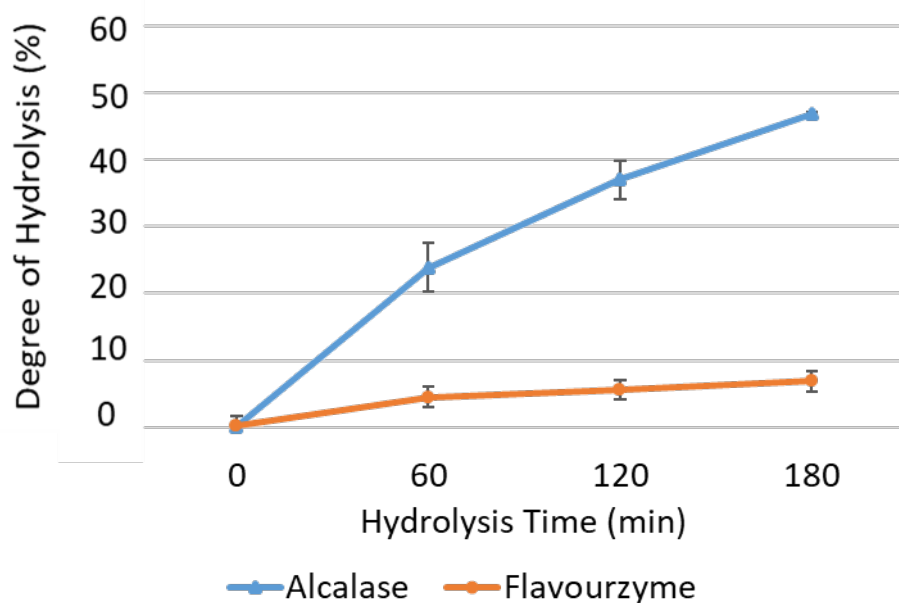
Fig. 4. Kinetics of the hydrolysis of S. almeriensis fresh biomass at 77 \text{ g}\cdot\text{kg}_{\text{SUS}}^{-1} by 3% (v.w) Alcalase or Flavourzyme. The experiment was performed in duplicate, error bars represent standard errors.
