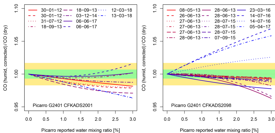
Figure 10. Ratios of CO (humid, corrected)/CO (dry) amount fractions vs. the water vapour mixing ratios of two different Picarro G2401 NIR-CRDS analysers over time. The legend shows the date (dd-mm-yy) of the experiment. The coloured areas are the limits for the WMO/GAW network compatibility goal (green) and extended (yellow) network compatibility goal at the amount fraction of 300 nmol mol -1 CO.
