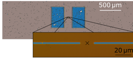
Figure 8.1: Transmon qubit chip False colored micrograph of the transmon qubit. The capacitor pads dominate the geometrical design of the structure, with only small connecting Al strips leading to the Josephson junction. The junction itself with an estimated size of 100 \times 95 \text{ nm}^2 is too small to be seen here even in the zoom-in and is only depicted schematically.
