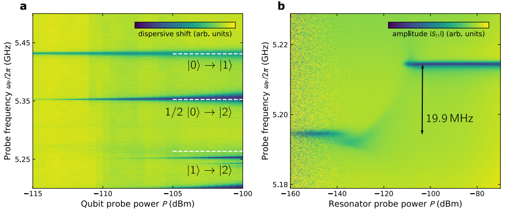
Figure 8.2: Spectroscopic measurements, qubit transitions and qubit-resonator coupling (a) The first transitions frequencies are obtained by evaluating the dips in the dispersive shift spectrum of the TE_{103} readout mode that is \Delta_{103}/2\pi = 1.14 GHz detuned from the qubit. The transition frequencies and the non-equidistant frequency spacing determine the characteristic qubit energies; E_J = 23.355 \text{ GHz} \cdot h , E_C = 167.8 \text{ MHz} \cdot h , and E_J/E_C = 139.2 . The calculated |1\rangle \rightarrow |2\rangle transition matches well with the corresponding signal. (b) The TE_{102} cavity mode (coupling mode) becomes dressed by the qubit presence (low power). At higher powers the qubit is saturated and the system decouples. The shift of nearly 20 MHz relates to a coupling between qubit and coupling mode of g_{q,102}/2\pi = 66.26 \text{ MHz} .
