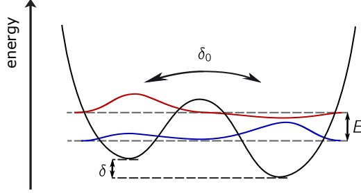
Figure 2.6: Double-well potential modeling a TLS The energy of the two states is given by the ground state energy difference \delta and the tunneling rate \delta_0 . The barrier can be overcome by thermal excitation or quantum tunneling.
