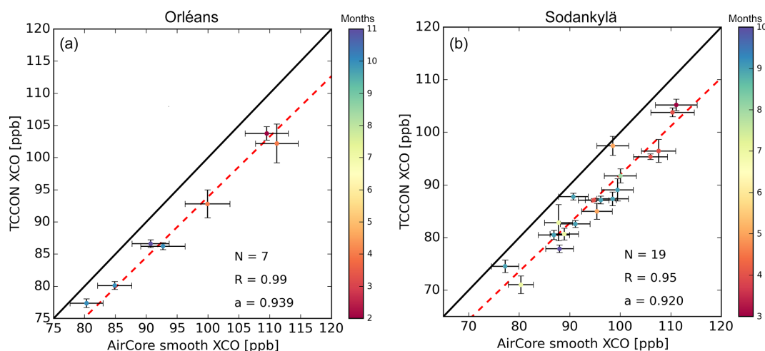
Figure 8. The scatter plots between the TCCON X CO retrievals and the smoothed AirCore X CO measurements at Orléans (a) and Sodankylä (b). The black line is the one-to-one line, and the red dashed line is the linear fitting (forced to cross the zero). The data are colored their measurement times in each month. The error bar of the TCCON X CO retrieval is the daily SD, representing the random uncertainty of the TCCON data, while the error bar of the AirCore data is the total uncertainty for each measurement. N is the number of co-located measurements, R is the correlation coefficient and a is the slope of the fitting line.
