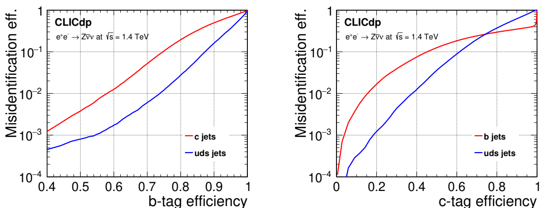
Figure 6. Flavour tagging performance in e^+e^- \rightarrow Z\bar{\nu}v events at 1.4 TeV reconstructed in the CLICdp detector. The fake rates for jets of other flavours are shown as functions of the b-tag (left) and c-tag (right) efficiencies.
