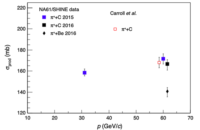
FIG. 4. Summary of production cross section measurements. The results are compared to previous results from NA61/SHINE [16] and Carroll et al. [22].
