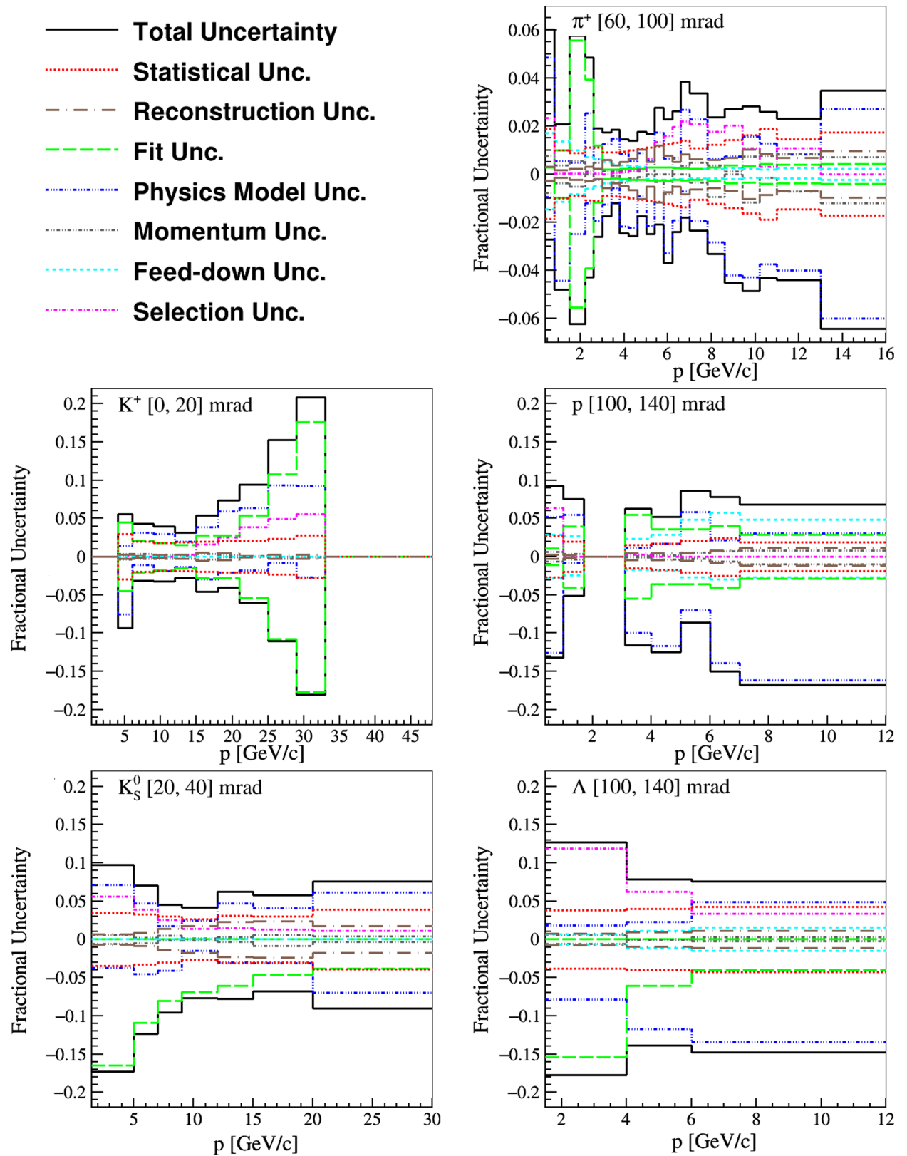
FIG. 12. The breakdown of the fractional uncertainties on \pi^+ , K^+ , proton, K_S^0 and \Lambda spectra from \pi^+ + C at 60 GeV/c interactions for select representative angular bins. The upper and lower uncertainties are shown on the positive and negative sides of the y axes.
