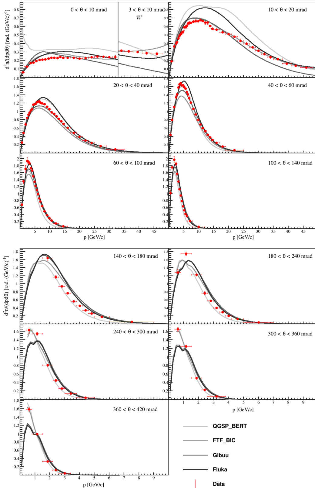
FIG. 16. \pi^+ multiplicity spectra from \pi^+ + C at 60 GeV/c interactions are shown. The error bars represent total uncertainties except for the normalization uncertainty. Note that the first angular bin ([0,10] mrad) is divided into two regions. For momenta less than 33 GeV/c, the angular range is [0,10] mrad and for momenta greater than 33 GeV/c, the angular range is [3,10] mrad. The results are compared to the predictions of the GEANT4 physics lists: QGSP_BERT and FTF_BIC as well as GiBUU2019 and FLUKA2011.
