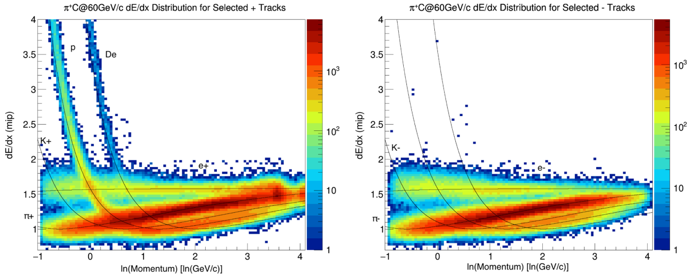
FIG. 10. Two-dimensional distributions of dE/dx and p are shown for the selected positively (left) and negatively (right) charged tracks in the \pi^+ + C at 60 GeV/c analysis. The black lines represent the Bethe-Bloch predictions for the dE/dx mean position of electrons, pions, kaons, protons and deuterons.
