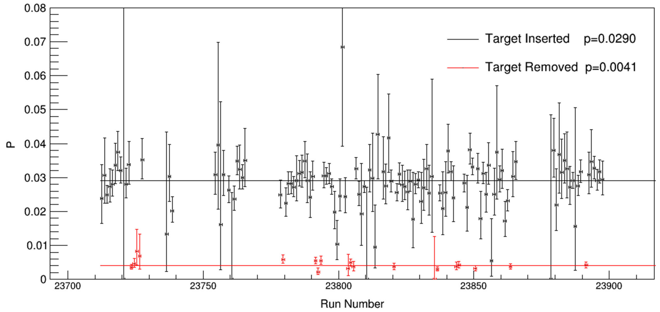
FIG. 3. Trigger interaction probabilities for the \pi^+ + C at 60 GeV/ c data set for target-inserted and target-removed runs.
