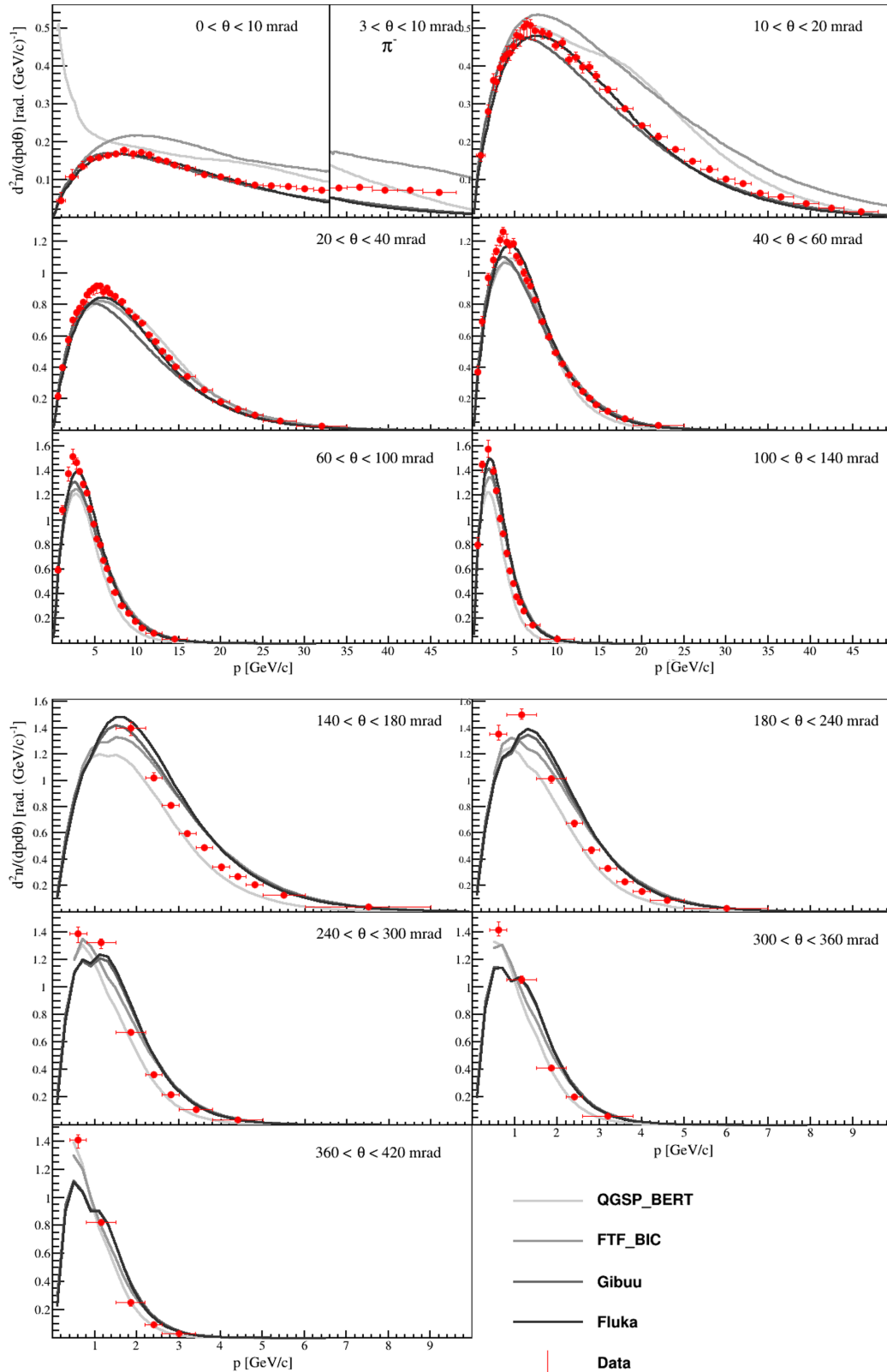
FIG. 17. \pi^- multiplicity spectra from \pi^+ + C at 60 GeV/c interactions are shown. The error bars represent total uncertainties except for the normalization uncertainty. Note that the first angular bin ([0,10] mrad) is divided into two regions. For momenta less than 33 GeV/c, the angular range is [0,10] mrad and for momenta greater than 33 GeV/c, the angular range is [3,10] mrad. The results are compared to the predictions of the GEANT4 physics lists: QGSP_BERT and FTF_BIC as well as GiBUU2019 and FLUKA2011.
