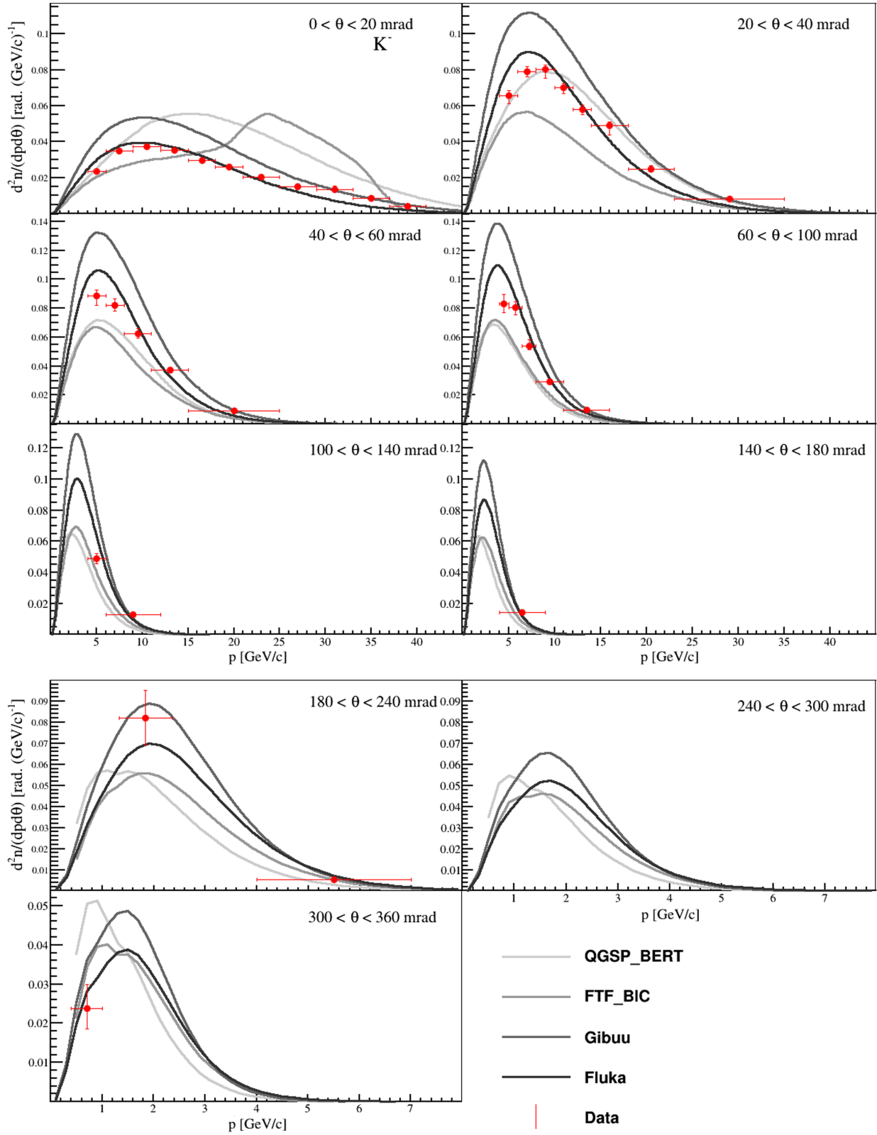
FIG. 19. K^- multiplicity spectra from \pi^+ + C at 60 GeV/c interactions are shown. The error bars represent total uncertainties except for the normalization uncertainty. The results are compared to the predictions of the GEANT4 physics lists: QGSP_BERT and FTF_BIC as well as GiBUU2019 and FLUKA2011.
