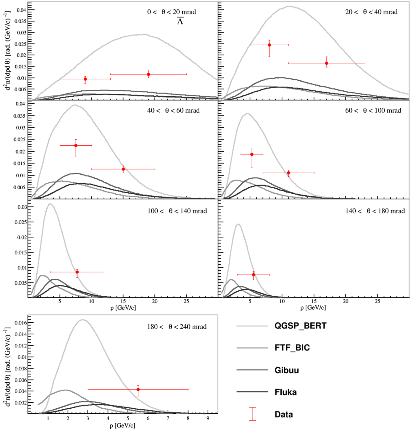
FIG. 15. \bar{\Lambda} multiplicity spectra from \pi^+ + C at 60 GeV/c interactions are shown for different regions of \theta . The error bars represent total uncertainties except for the normalization uncertainty. The results are compared to the predictions of the GEANT4 physics lists: QGSP_BERT and FTF_BIC as well as GiBUU2019 and FLUKA2011.
