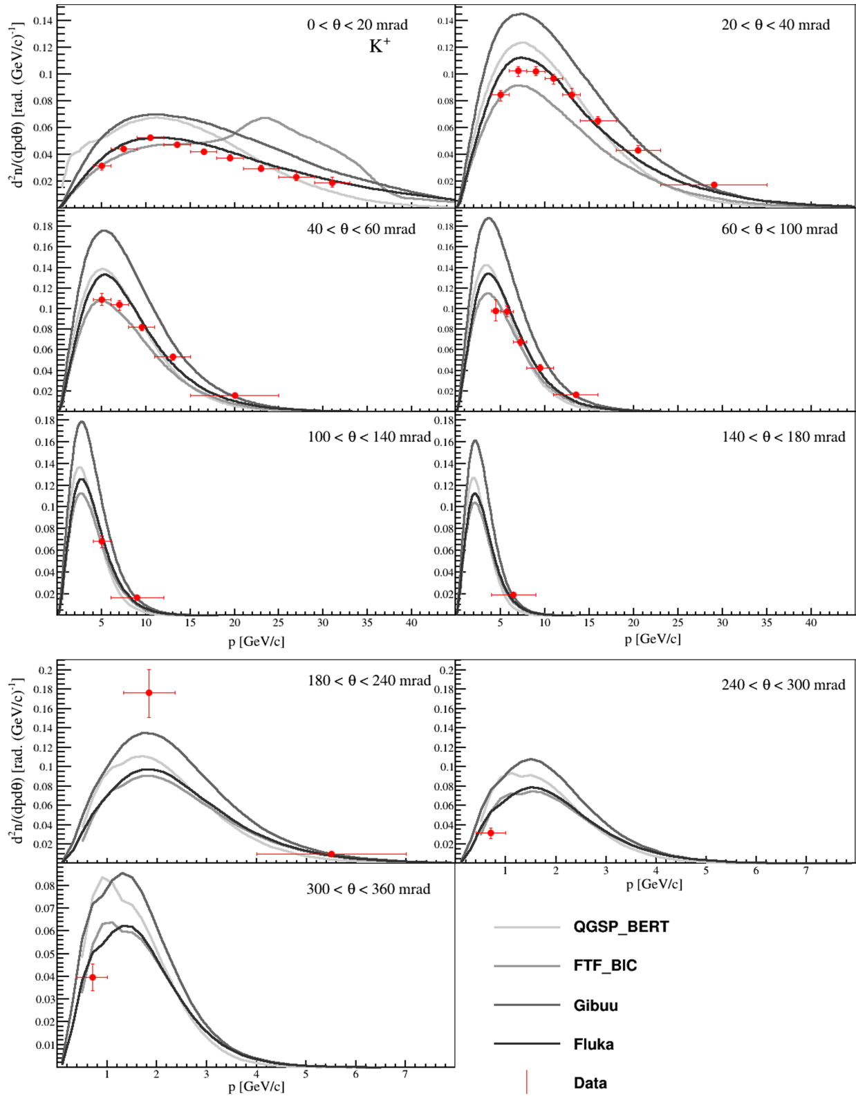
FIG. 18. K^+ multiplicity spectra from \pi^+ + C at 60 GeV/c interactions are shown. The error bars represent total uncertainties except for the normalization uncertainty. The results are compared to the predictions of the GEANT4 physics lists: QGSP_BERT and FTF_BIC as well as GiBUU2019 and FLUKA2011.
