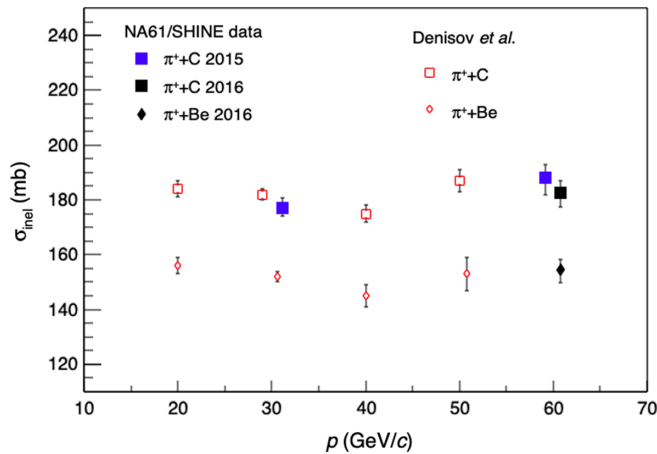
FIG. 5. Summary of inelastic cross section measurements. The results are compared to previous results from NA61/SHINE [16] and Denisov et al. [23].
