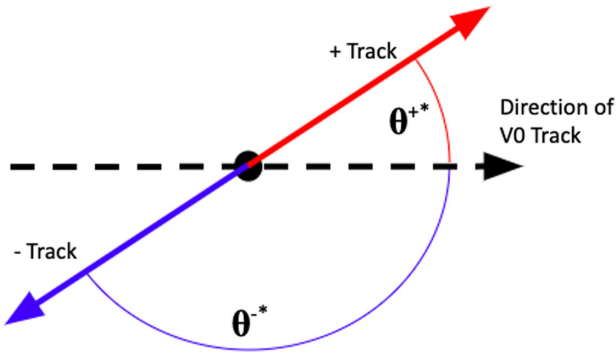
FIG. 6. This cartoon shows the relevant angles in V^0 decays in the rest frame of the V^0 . The child particles decay back to back in this frame. The angle at which the positively charged particle is emitted is \theta^{+*} , and the angle at which the negatively charged particle is emitted is \theta^{-*} .
