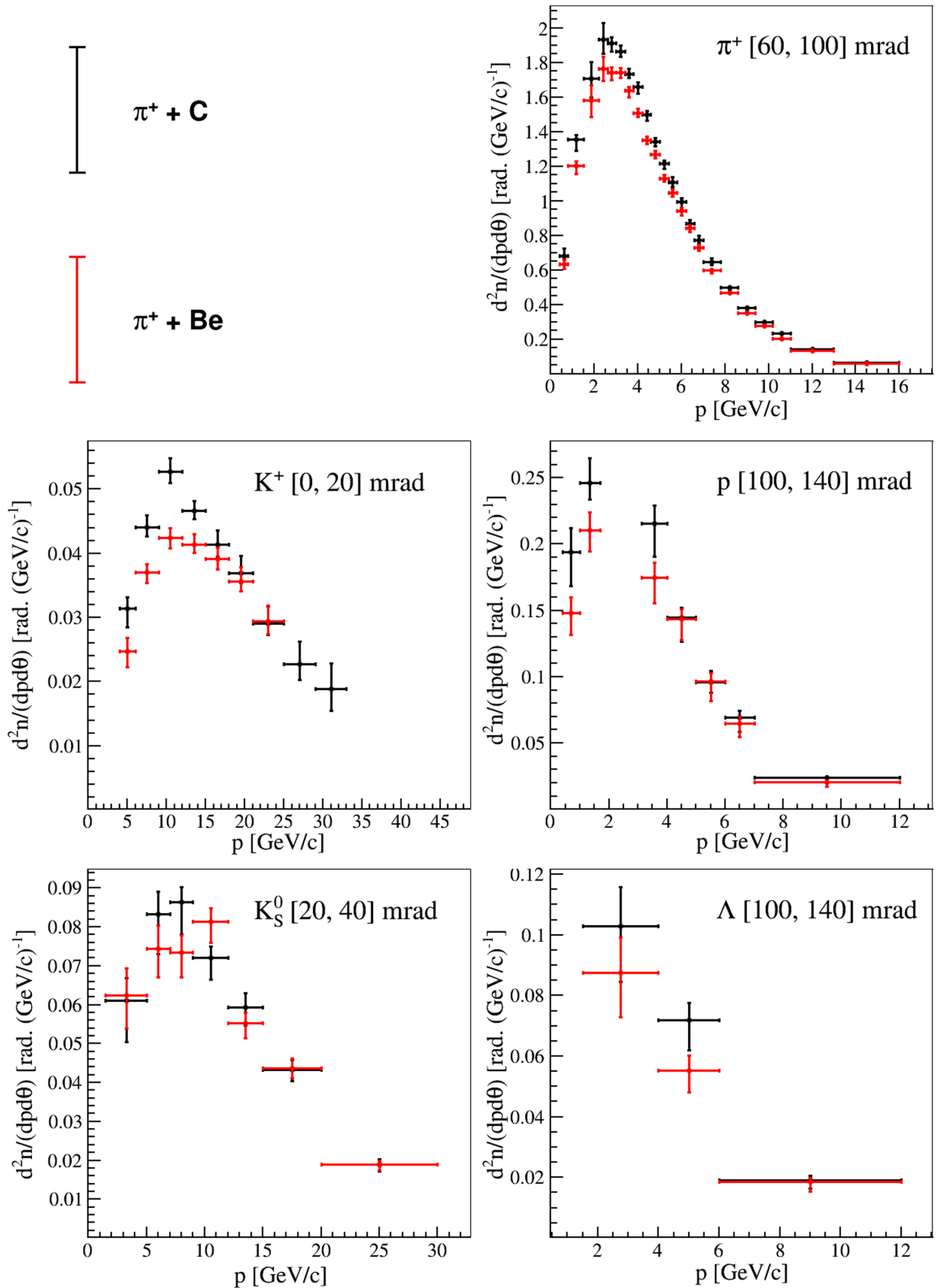
FIG. 21. Measurements of spectra from \pi^+ + C at 60 GeV/c and \pi^+ + Be at 60 GeV/c interactions are shown for produced \pi^+ , K^+ , proton, K_S^0 and \Lambda for select representative angular bins. The error bars represent total uncertainties except for the normalization uncertainty.
