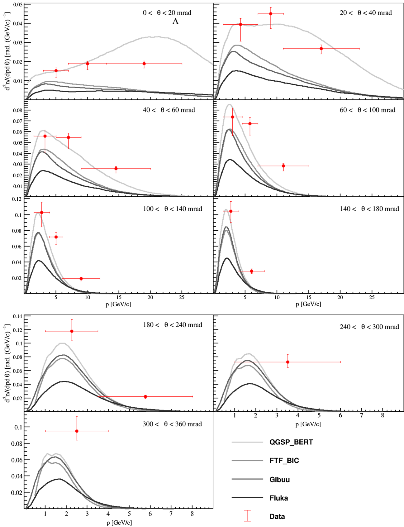
FIG. 14. \Lambda multiplicity spectra from \pi^+ + C at 60 GeV/c interactions are shown for different regions of \theta . The error bars represent total uncertainties except for the normalization uncertainty. The results are compared to the predictions of the GEANT4 physics lists QGSP_BERT and FTF_BIC as well as GiBUU2019 and FLUKA2011.
