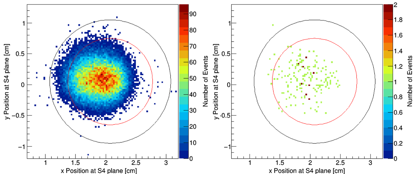
FIG. 2. Positions of BPD tracks extrapolated to the S4 plane in target-removed data runs from the \pi^+ + C at 60 GeV/ c data set. The measured S4 position is shown as a black circle and the BPD radius cut is shown as a red circle in both figures. Left: Events taken by the beam trigger. Right: Events taken by the interaction trigger.
