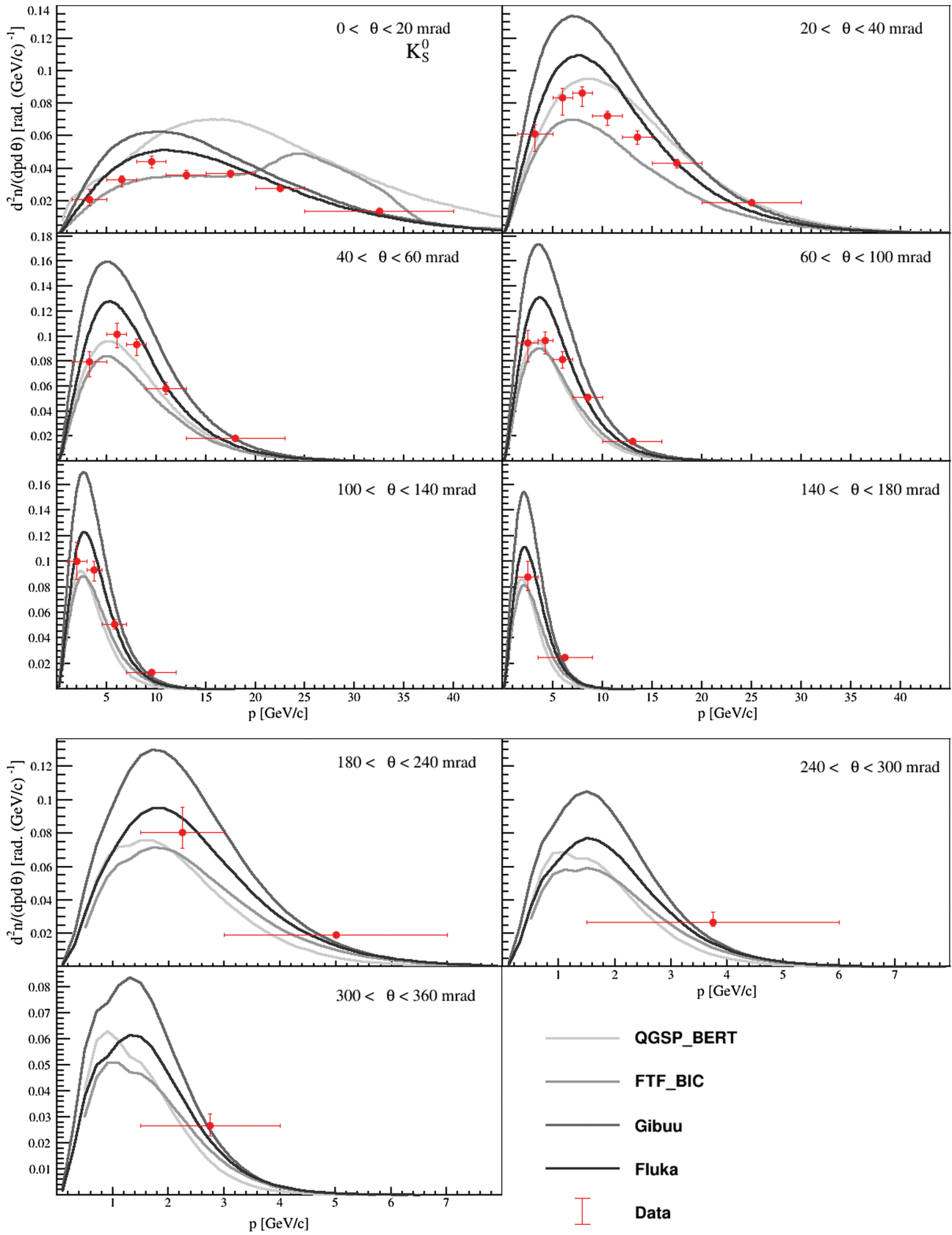
FIG. 13. K_S^0 multiplicity spectra from \pi^+ + C at 60 GeV/c interactions are shown for different regions of \theta . The error bars represent total uncertainties except for the normalization uncertainty. The results are compared to the predictions of the GEANT4 physics lists QGSP_BERT and FTF_BIC as well as GiBUU2019 and FLUKA2011.
