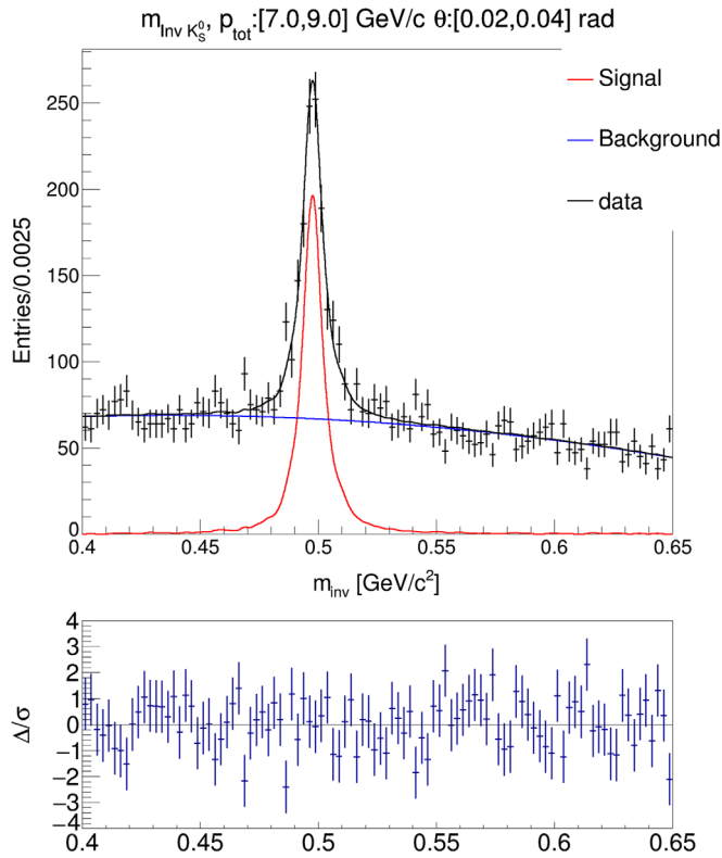
FIG. 8. Example fit to the K_S^0 invariant mass distribution in \pi^+ + C at 60 GeV/c data for an example kinematic bin. The m_{\text{inv}} distribution and the fitted model is shown in the top. The residuals of the fit are shown on the bottom.
