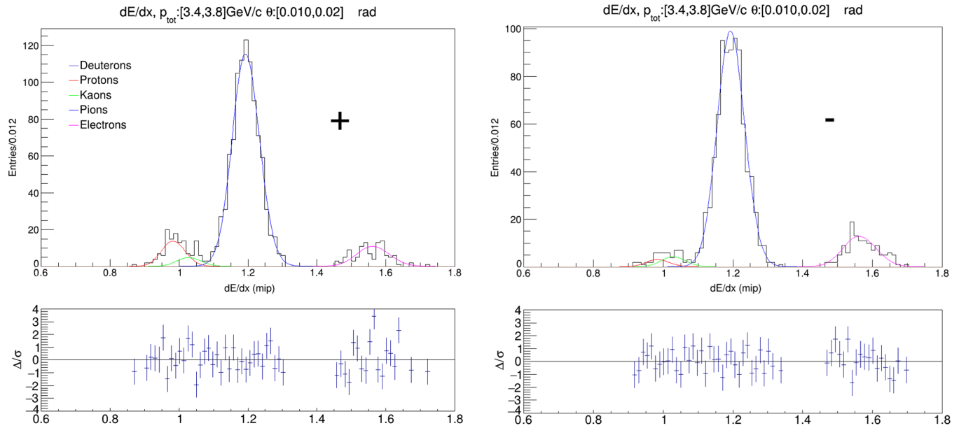
FIG. 11. An example fit to a dE/dx distribution is shown for the analysis of pions. On the top, the dE/dx distributions are shown for positively charged tracks (left) and negatively charged tracks (right) along with the fitted contributions due to the five particle species considered. On the bottom, the residuals of the fit with respect to the dE/dx distribution are shown.
