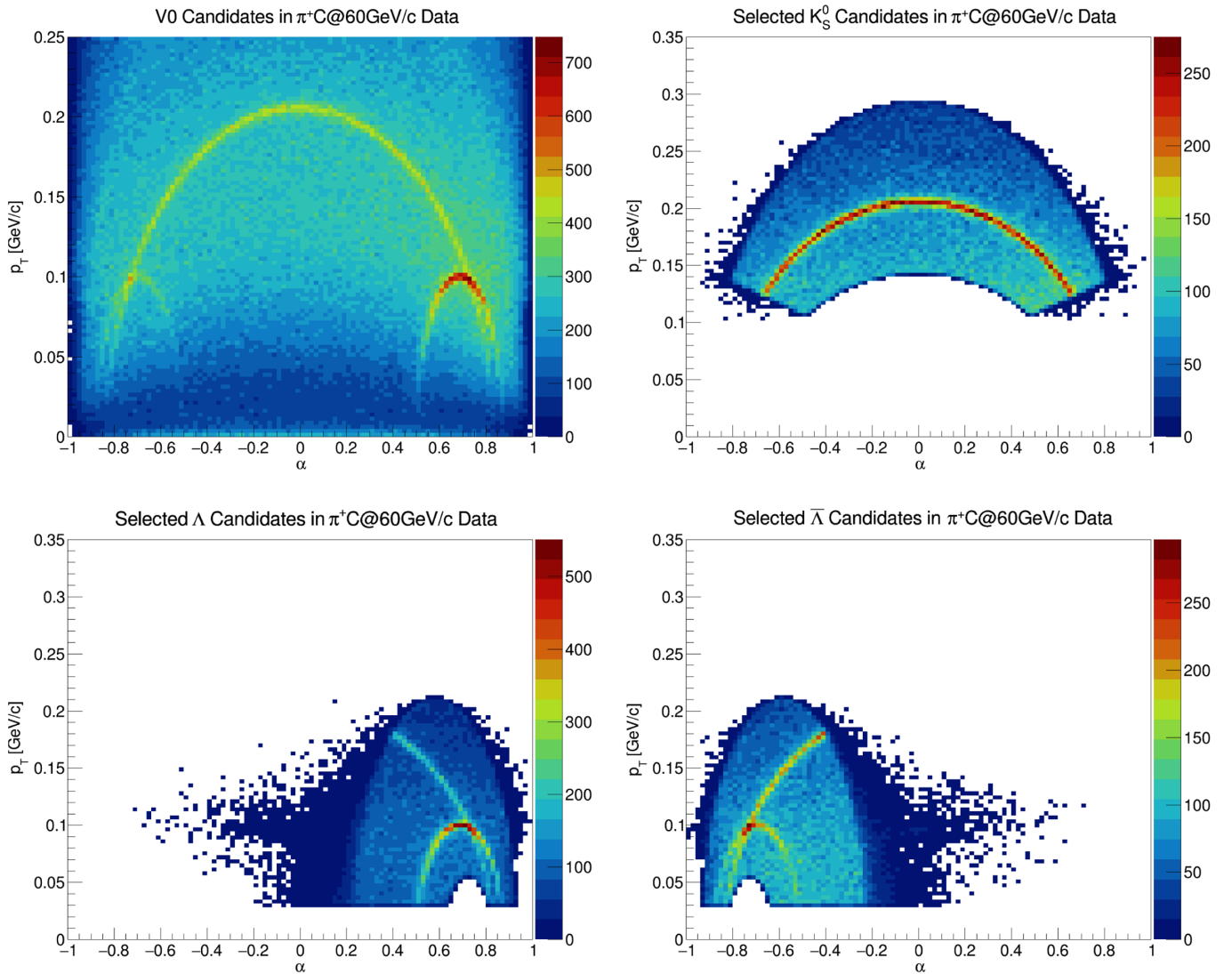
FIG. 7. The Armenteros-Podolansky distribution of the V^0 candidates in the \pi^+ + C at 60 GeV/c analysis before selection cuts were applied is shown in the top left. The distribution is shown after selection cuts are applied for the K_S^0 analysis (top right), \Lambda analysis (bottom left) and \bar{\Lambda} analysis (bottom right).
