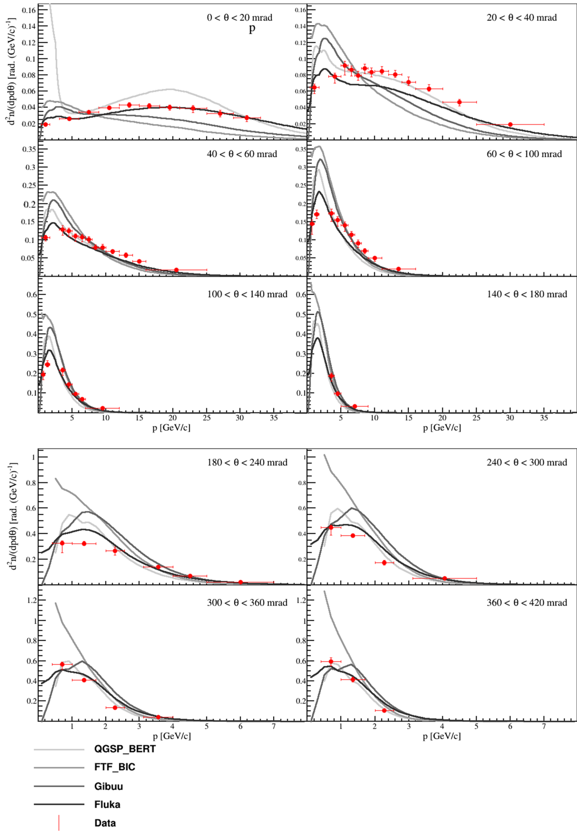
FIG. 20. Proton multiplicity spectra from \pi^+ + C at 60 GeV/c interactions are shown. The error bars represent total uncertainties except for the normalization uncertainty. The results are compared to the predictions of the GEANT4 physics lists: QGSP_BERT and FTF_BIC as well as GiBUU2019 and FLUKA2011.
