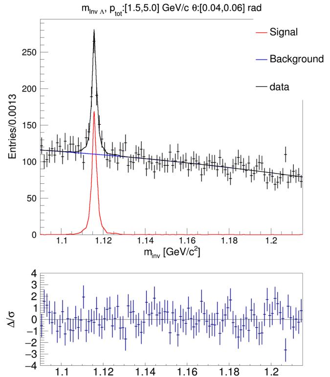
FIG. 9. Example fit to the \Lambda invariant mass distribution in \pi^+ + C at 60 GeV/c data for an example kinematic bin. The m_{\text{inv}} distribution and the fitted model is shown on the top. The residuals of the fit are shown on the bottom.
