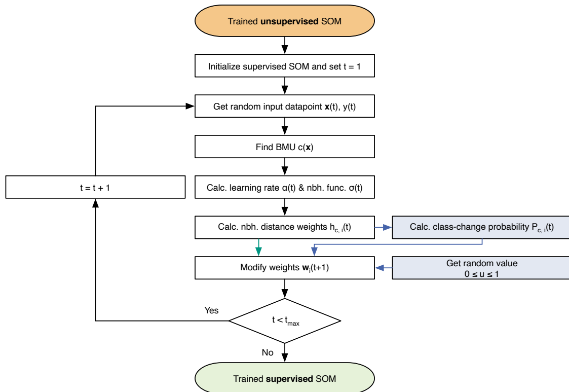
Figure 5. Flowchart of the algorithms for the regression SOM (black and cyan) and the classification SOM (black and blue). The “Trained unsupervised SOM” (orange) is the result of the unsupervised SOM algorithm illustrated in Figure 3.
