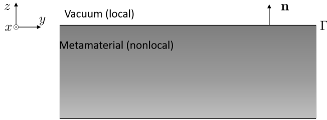
Figure 1: Illustration of the domain in which the light propagates, the upper-half space is occupied by vacuum and the lower-half space is occupied by a homogenized MM. The surface separating the two half-spaces is denoted \Gamma . The normal \mathbf{n} is outward directed from the homogenized MM.
