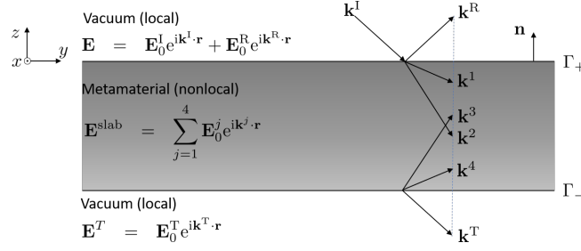
Figure 2: Propagating modes inside a slab MM. We have two forward modes defined on the the surface \Gamma^+ and the other backward modes are defined on the surface \Gamma^- .
