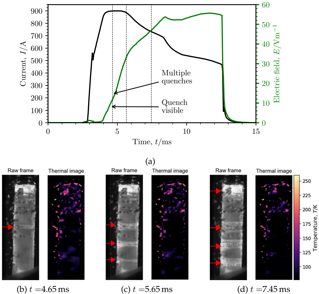
Figure 4.10.: Sample 3 pulsed with a 900 A, 12 ms long pulse. (a) shows the applied current pulse and the recorded electric field across the tape. (b)-(d) show raw and thermal images corresponding to times indicated by the black vertical lines in (a). The red arrows indicate the quench nucleation positions.
