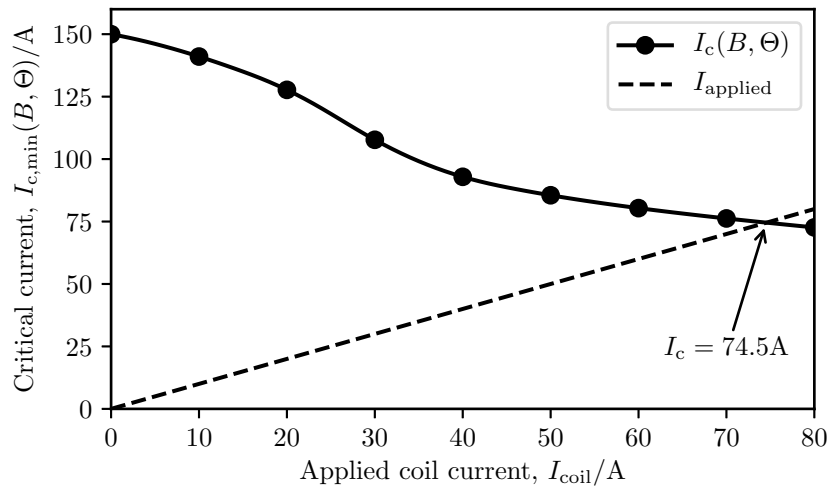
Figure 5.3.: Critical current search results using FEM simulation in the insulated coil. The curve shows the critical current of the coil as a function of the magnetic field, generated by the applied current as shown by the dashed line. The intersection of the two curves indicates the critical current of the coil.
