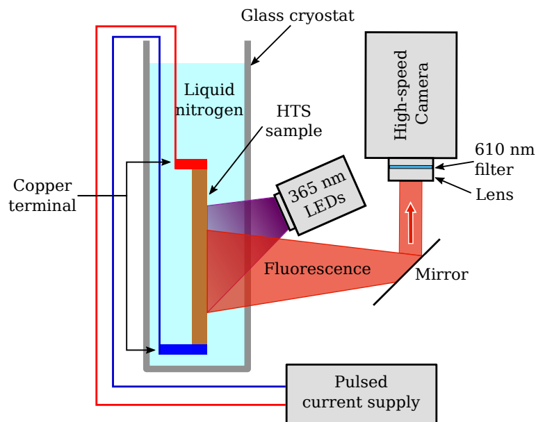
Figure 3.3.: Cross-section schematic view of the experimental assembly. The sample is placed in a double-walled glass cryostat and submerged in liquid nitrogen. The UV LED array excites the sample at an oblique angle and the high-speed camera records the fluorescent light emission through a mirror due to the experimental arrangement.
