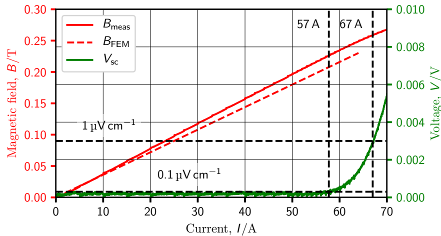
Figure 5.15.: Initial I_c measurement of the NI coil showing the 0.1 \mu\text{V cm}^{-1} and 1 \mu\text{V cm}^{-1} electric field criterion. The critical current of the coil is then 57 A and 67 A, respectively. The plot shows data points extracted from the measurement and not the actual ramping plot.
