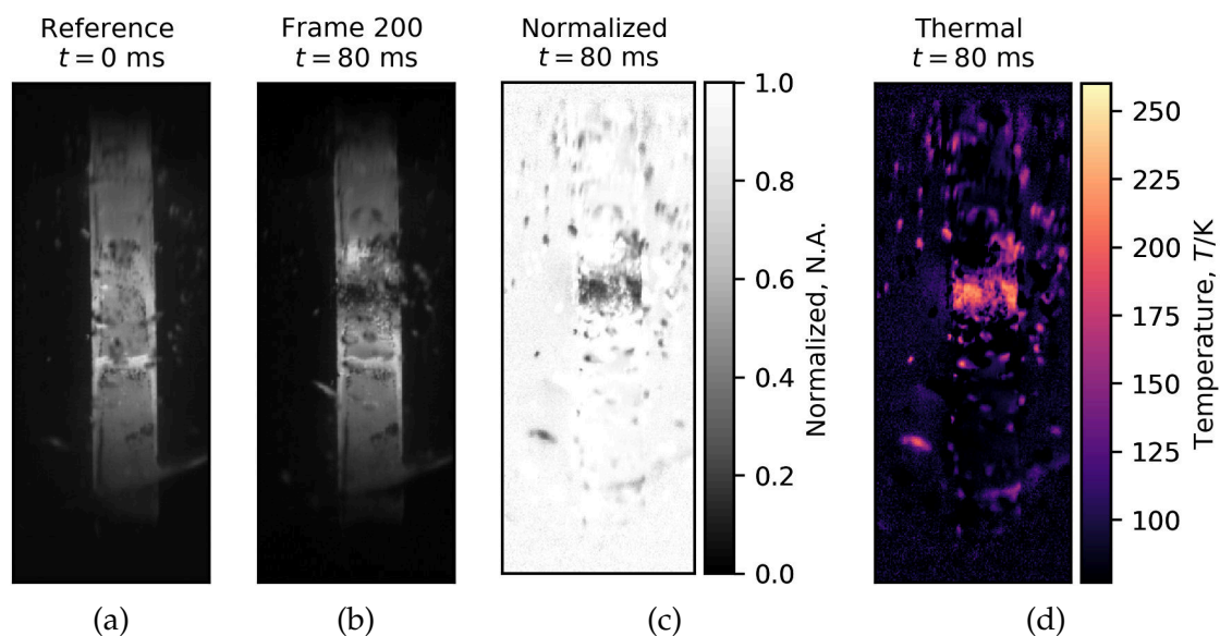
Figure 3.11.: Post-processing steps illustrated on an EuTFC coated HTS sample measurement. (a) shows a reference image. (b) shows frame 200 of the recording at 80 ms where some heating takes place at the centre of the sample. (c) shows frame 200 normalized with the reference frame. (d) shows the extracted thermal data from (c) using the calibration curve shown in Figure 3.10.
