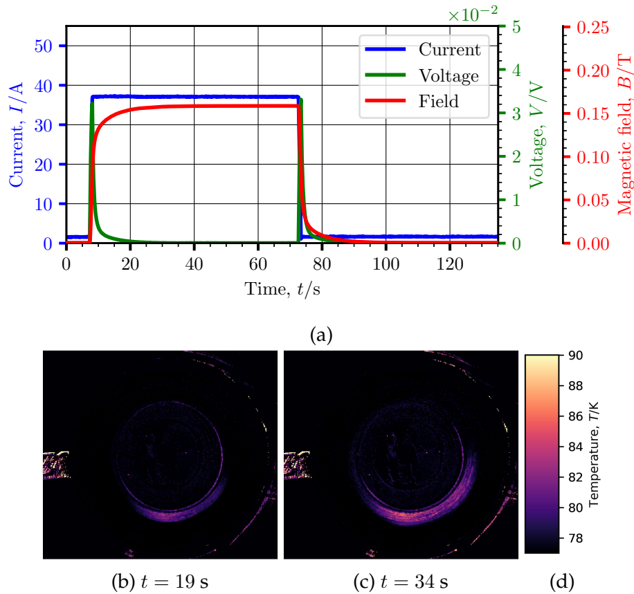
Figure 5.20.: Electrical and thermal effects of 50 \text{ A s}^{-1} ramping rate to 40 A.
