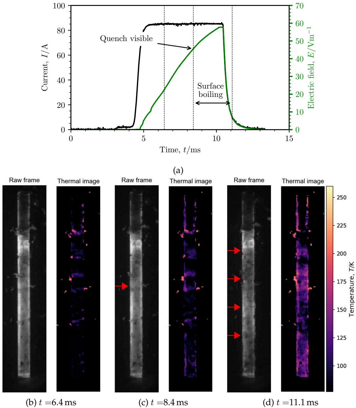
Figure 4.16.: Sample 6 (with a CFD architecture added at Polytechnique Montréal [18]) pulsed with a 85 A, 8 ms long pulse. (a) shows the applied current pulse and the recorded electric field across the tape. (b)-(d) show raw and thermal images corresponding to times indicated by the black vertical lines in (a). The red arrows indicate the quench development.
