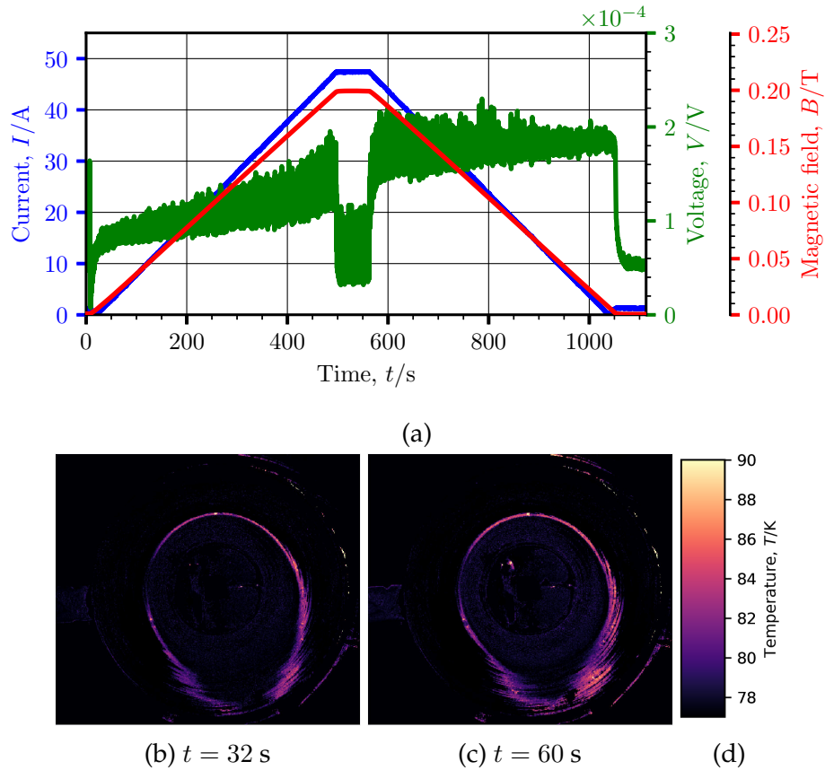
Figure 5.22.: Electrical and thermal effects of 0.1 \text{ A s}^{-1} ramping rate to 50 A.
