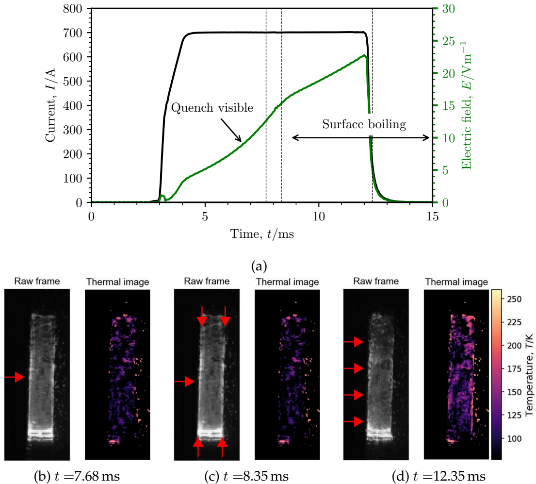
Figure 4.13.: Sample 9 pulsed with a 700 A, 12 ms long pulse. (a) shows the applied current pulse and the recorded electric field across the tape. The arrows show the point where the quench is first visible on the thermal imaging recording and where multiple quench zones started forming. (b)-(d) show raw and thermal images corresponding to times indicated by the black vertical lines in (a). The red arrows indicate the quench development.
