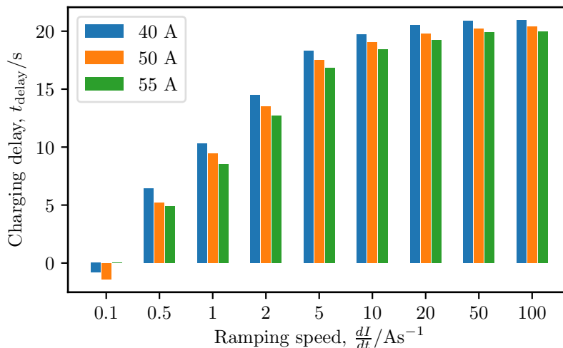
Figure 5.23.: Charging delay t_{\text{delay}} of the NI coil as a function of ramping rates between 0.1 \text{ A s}^{-1} to 100 \text{ A s}^{-1} . Data for the 0.1 \text{ A s}^{-1} ramping rate to 55 A is missing.
