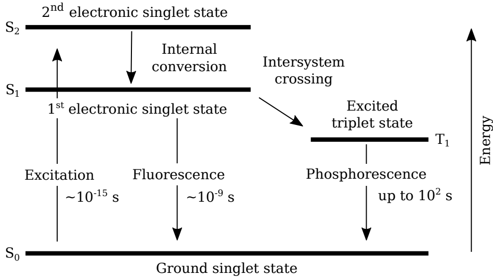
Figure 3.4.: Simplified diagram showing the mechanics of excitation, fluorescence and phosphorescence including the representative duration of these effects. The figure only shows internal conversion between electronic states and intersystem crossing from singlet to triplet state, vibrational relaxation within the electronic levels is not shown.
