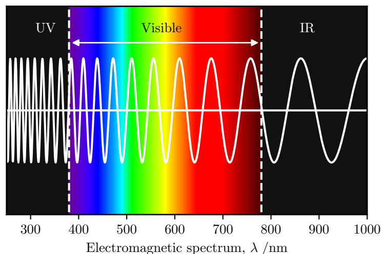
Figure 3.1.: Representation of the electromagnetic spectrum between wavelengths of 250 nm (near ultraviolet, UV) and 1 \mu\text{m} (near-infrared, IR). The spectrum visible for the human eye between approximately 380 nm and 780 nm is highlighted and shown with the colours matching the wavelengths.
