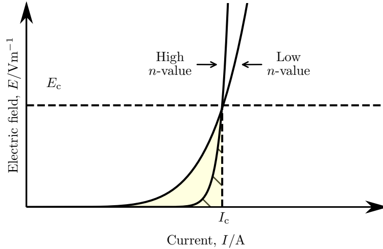
Figure 2.6.: Definition of the critical current in superconductors using the E_c criterion and the importance of the n -value. While the conductors have an identical critical current, the one with a lower n -value will develop an electrical field sooner and hence incur I^2R losses as indicated by the shaded areas.
