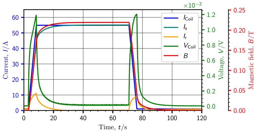
Figure 5.18.: Time development of measured current, voltage and magnetic field in the non-insulated coil when ramped at 10 \text{ A s}^{-1} to 55 A. The radial and the spiral current ( I_r , I_s ) were calculated using eq. 5.15.
