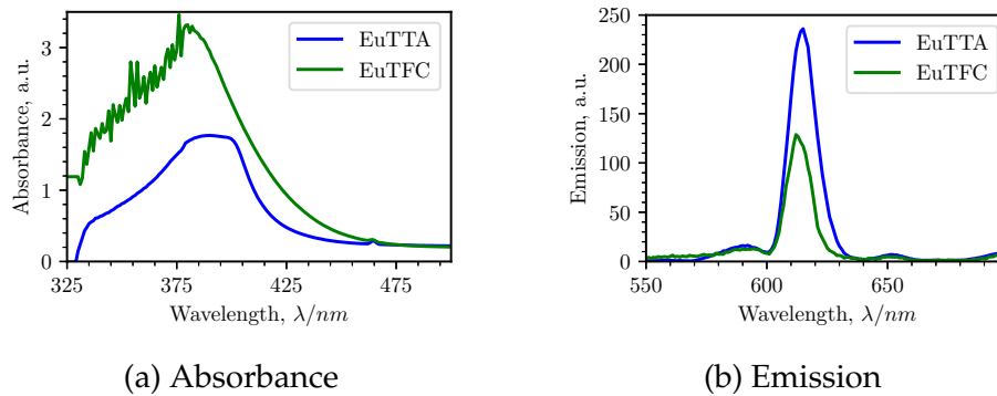
Figure 3.5.: Measured (a) absorbance and (b) emission spectra of EuTTA and EuTFC in a polymethyl methacrylate solution at room temperature [99]. (a) shows an absorption of over 90 % of the incoming light between 340 nm and 400 nm for both compounds. In (b) the principal emission peak at 612 nm is visible when using 380 nm excitation light.
