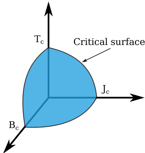
Figure 2.2.: A superconductor will remain superconducting as long as it stays below its critical temperature, current density and magnetic flux density. The superconducting region is shown by the coloured area in the figure.
