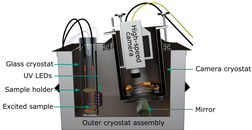
Figure 4.1.: Cross-section view of the experimental assembly for HTS tape measurements. A larger cryostat bath is used as an outer enclosure, holding a double-walled glass cryostat, a submersible, cylindrical cryostat for the high-speed camera as well as the camera itself.
