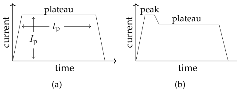
Figure 4.3.: Direct current pulse shapes applied to HTS tapes. (a) shows a rectangular current pulse. (b) shows a rectangular current pulse, with an initial peak at a higher amplitude for a short duration.
