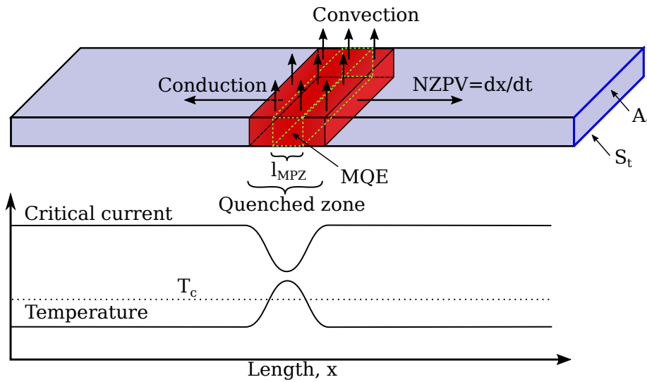
Figure 2.7.: Concepts of quench, normal zone propagation, minimum quench energy and minimum propagation length in a HTS coated conductor cooled in a cryogenic bath. The arrows represent heat transfer by different mechanisms, whereas the bottom plot illustrates the critical current density and temperature profile of the tape.
