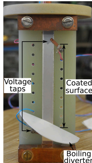
Figure 4.2.: Close-up of the sample holder showing a 12 mm stabilizer-free sample placed at the centre with two voltage taps. The approximated length of the surface with the fluorescent coating as well as the “boiling diverter” are shown.
