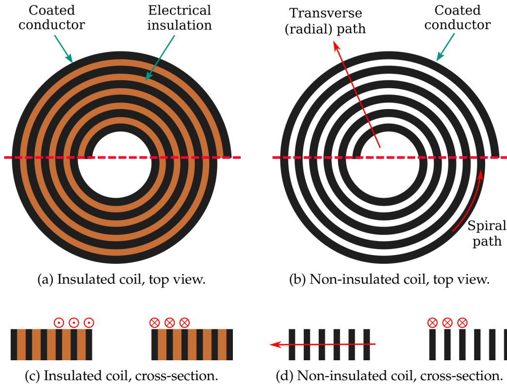
Figure 2.9.: Concept drawing of an insulated coil (a) and a non-insulated coil (b), with corresponding cross-sections shown across the red dashed line in (c) and (d), respectively. The red arrows indicate possible current paths.
