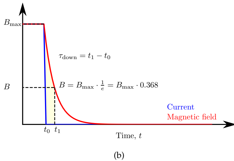
Figure 2.11.: Concepts of various time constants. (a) shows the charging time constant \tau_{\text{up}} in the hatched area and the charging delay t_{\text{delay}} in the coloured area. (b) shows the discharge time constants \tau_{\text{down}} in the coloured area. The features of the plots are exaggerated for visualization.
