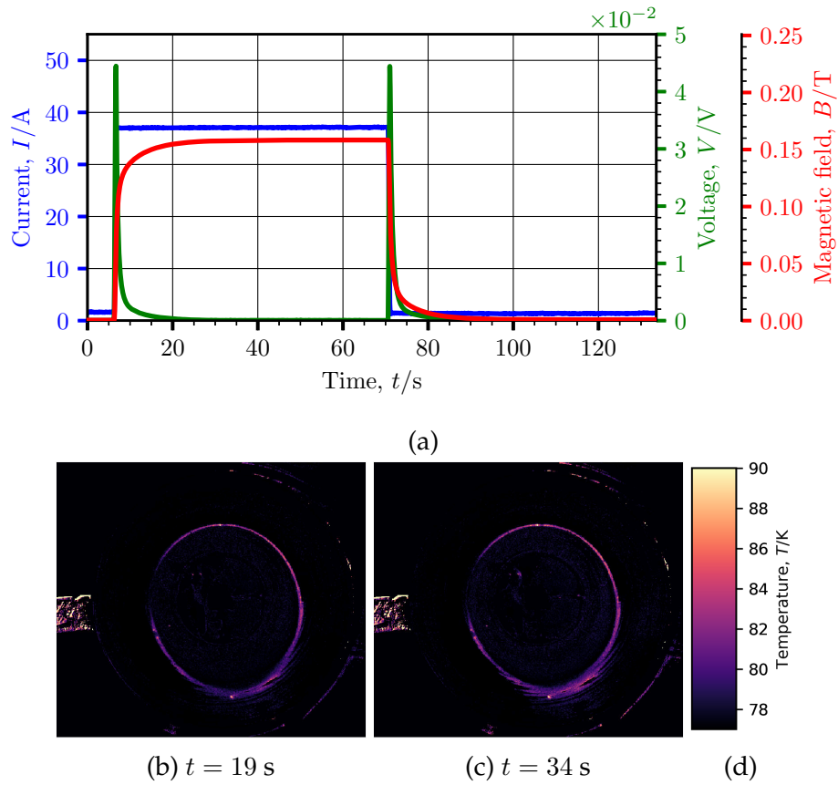
Figure 5.21.: Electrical and thermal effects of 100 \text{ A s}^{-1} ramping rate to 40 A.
