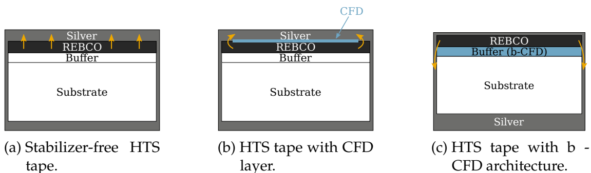
Figure 4.14.: Cross-section of various HTS tape architectures. Subfigure (a) shows a common HTS tape, with uniform inter-facial resistance, (b) shows the CFD architecture with an artificially increased inter-facial resistance and (c) shows the b-CFD concept where the thickness of the Ag stabilization is changed on the front- and back-side of the tape [47]. The arrows indicate current sharing paths.
