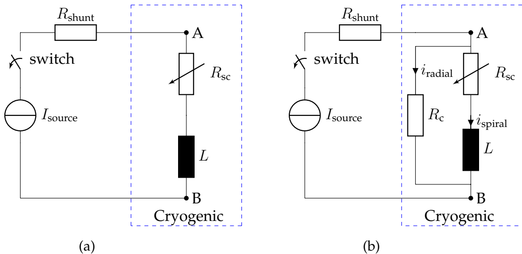
Figure 2.10.: Simplified circuit diagrams for (a) an insulated HTS coil and (b) a non-insulated HTS coil also showing the cryogenic environment. The coil voltage is measured between points A and B.
