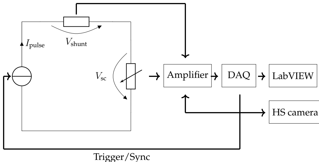
Figure 4.4.: Data acquisition of various voltage signals in the pulsed quench measurements.
