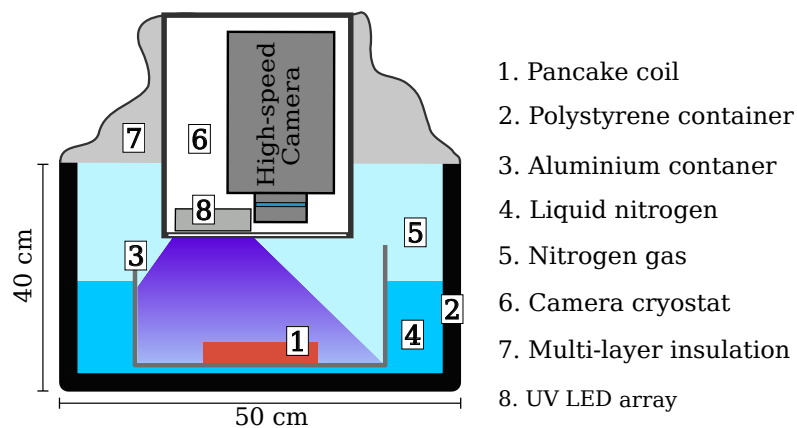
Figure 5.5.: Cross-section drawing of the coil measurement assembly. The coil is fixed with thermal paste at the bottom of the aluminium container and excited by the UV LEDs from inside a separate cryostat housing the high-speed camera. Radiation heat load and ambient light are blocked by sheets of multi-layer insulation.
