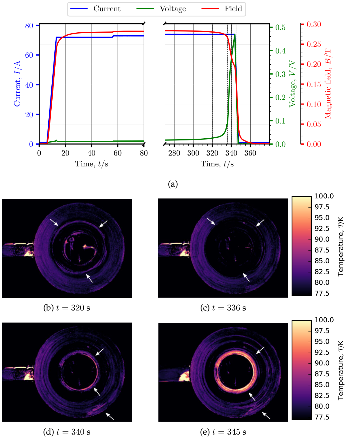
Figure 5.27.: Electrical and thermal measurement results of the 74 A overcurrent measurement. Dashed lines indicate positions of thermal images. (a) shows the time development of the applied current ramp, coil voltage and magnetic field. (b)-(e) show thermal images, where white arrows indicate specific features.
