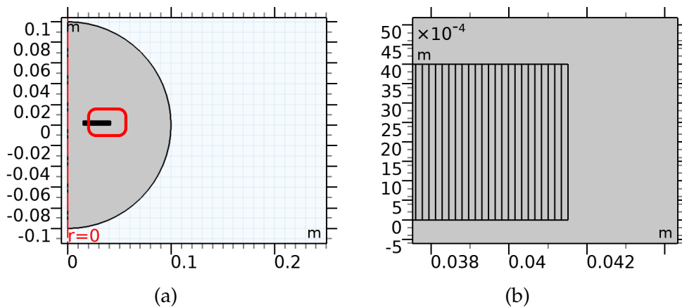
Figure 5.1.: (a) shows a cross-section view of the coil turns and the air domain around it, where r is axis of symmetry. (b) shows a zoomed view of the of the coil geometry as highlighted by the red rectangle in (a), where each thin strip represents a turn of the pancake coil.
