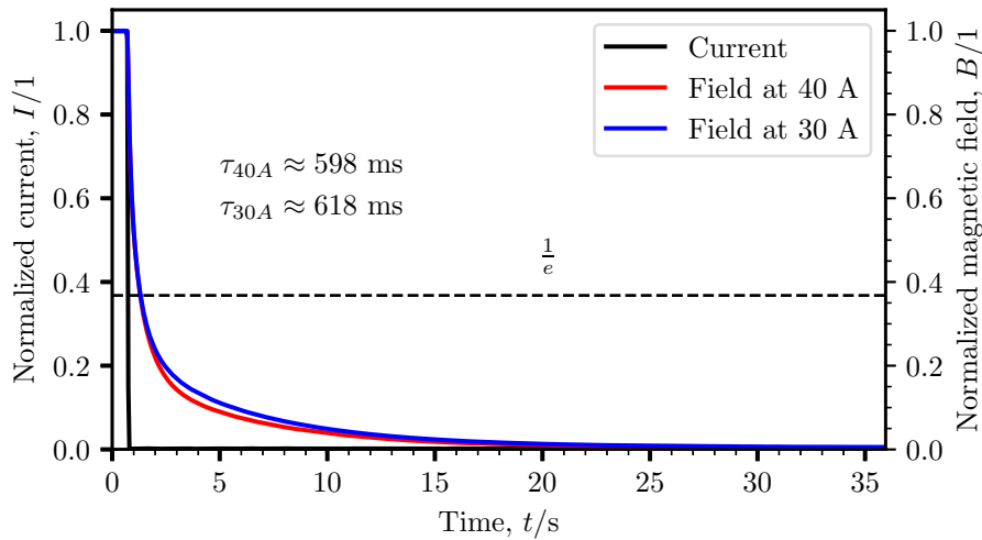
Figure 5.25.: Normalized magnetic field development during sudden discharge tests at steady DC current levels of 30 A and 40 A. The dashed line indicates the 0.37 criterion where the time constant is evaluated.
