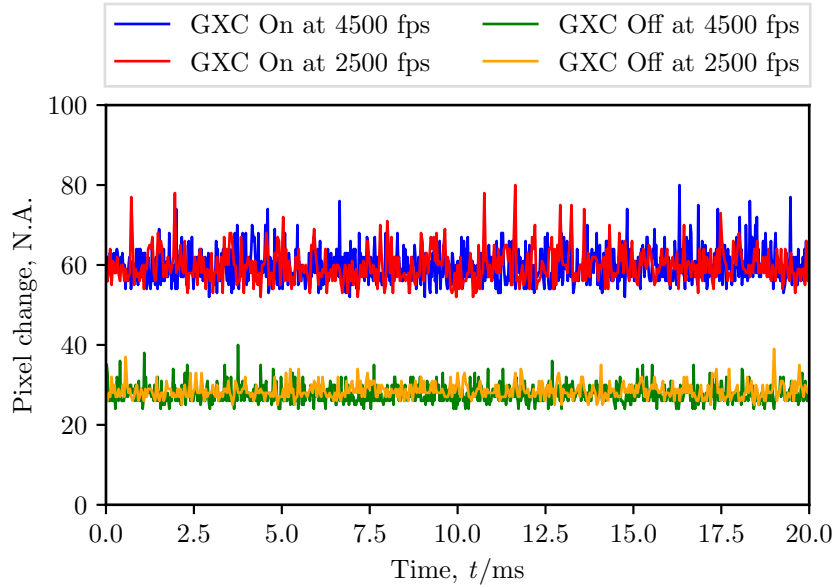
Figure 3.14.: Time evolution of dark noise in the camera with closed shutter at two distinct recording rates with and without GXC. The levels represent the single largest change of recorded light intensity of any pixel with respect to its prior state.
