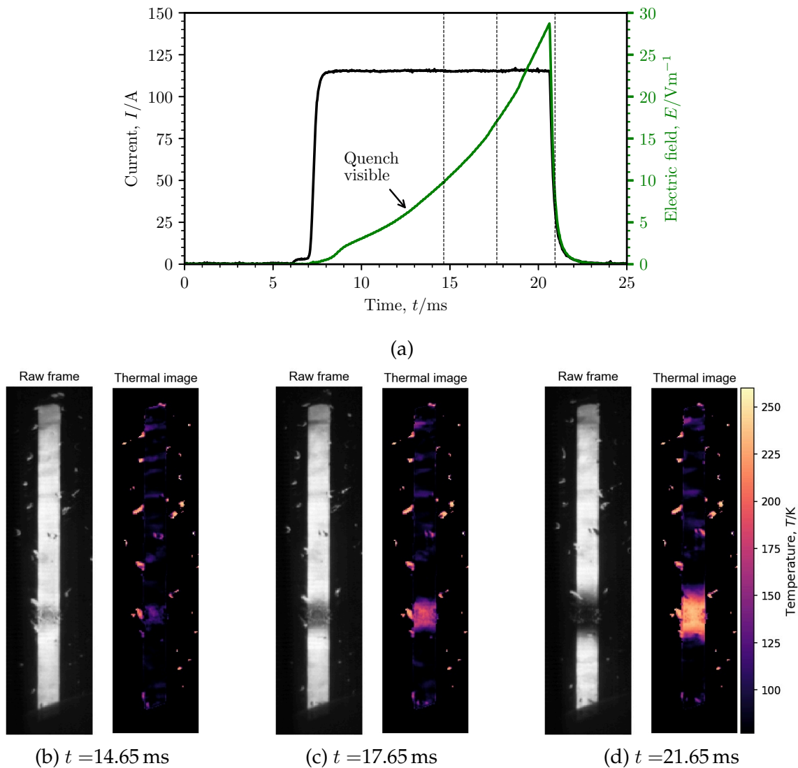
Figure 4.8.: Sample 4 pulsed with a 115 A, 12 ms long pulse. (a) shows the applied current pulse and the recorded electric field across the tape. (b)-(d) show raw and thermal images corresponding to times indicated by the black vertical lines in (a).
