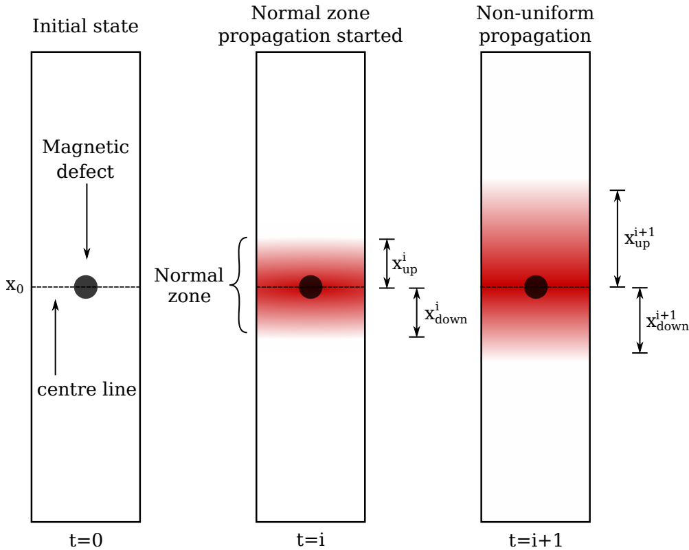
Figure 4.5.: Normal zone propagation in HTS tapes showing the steady-state operation at 77 K as well as two time instances after the appearance of a normal zone. The red coloured area indicates the propagation of the 93 K front, used as a criterion for calculating the NZPV.
