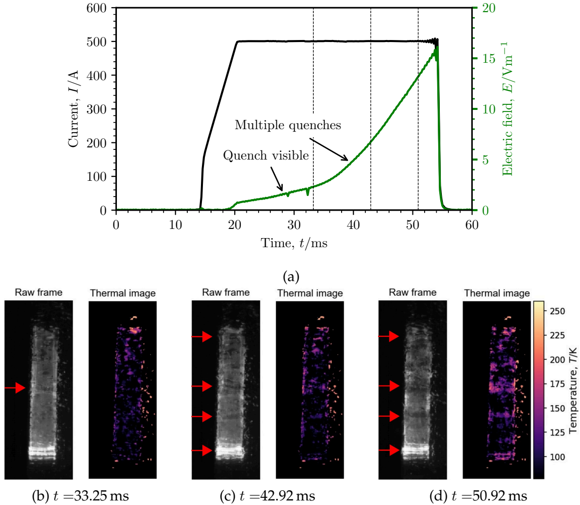
Figure 4.12.: Sample 9 pulsed with a 500 A, 50 ms long pulse. (a) shows the applied current pulse and the recorded electric field across the tape. The arrows show the point where the quench is first visible on the thermal imaging recording and where multiple quench zones started forming. (b)-(d) show raw and thermal images corresponding to times indicated by the black vertical lines in (a). The red arrows indicate the quench nucleation positions.
