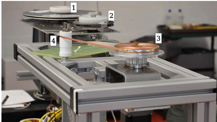
Figure 5.9.: Picture of the winding machine assembly, highlighting: (1) the source spool of the 4 mm HTS tape, (2) the spool of Kapton ® being co-wound with the HTS tape and (3) the target coil. Both tapes were passed through a nylon cylinder (4) to keep them aligned during winding.
