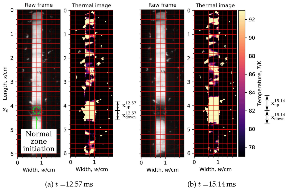
Figure 4.6.: Example of a recording post-processed for calculating the normal zone propagation velocity. (a) shows the normal zone at time 12.57 ms and (b) at 15.14 ms. Both show the raw frame (left) and a thermal image (right), with a scale boundaries between 77 K to 93 K. The red grid lines are 2 mm apart and the arrows indicate the nucleation point (caused by the magnetic defect) and the distance travelled by the quench in the up- and downwards direction.
