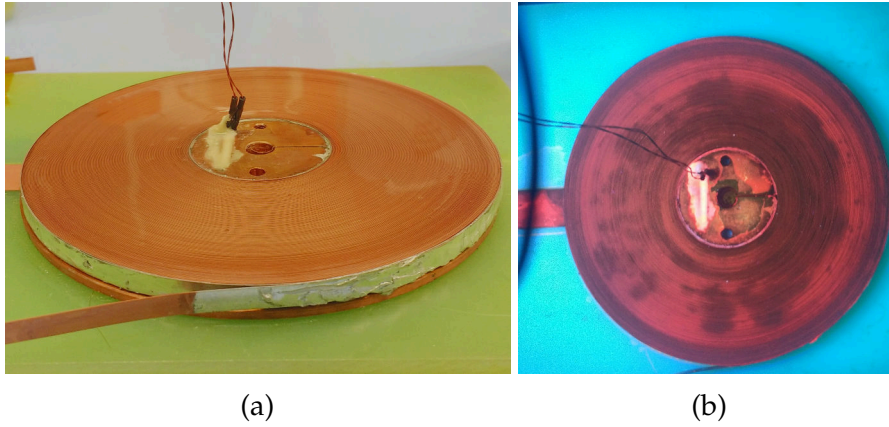
Figure 5.14.: (a) shows the NI coil's surface completely covered with the coating solution. In (b) the fluorescent emission from the coating shows a strong non-uniformity and partially missing spots.
