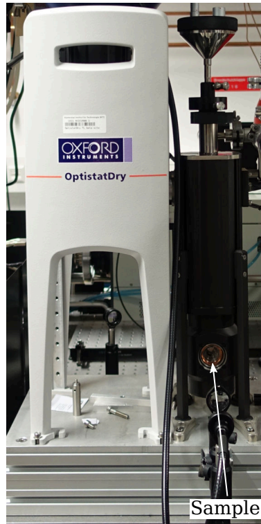
Figure 3.8.: Optistat Dry cryostat used for calibrating the temperature dependant fluorescence in the EuTFC and EuTTA samples from 4 K to 300 K.
