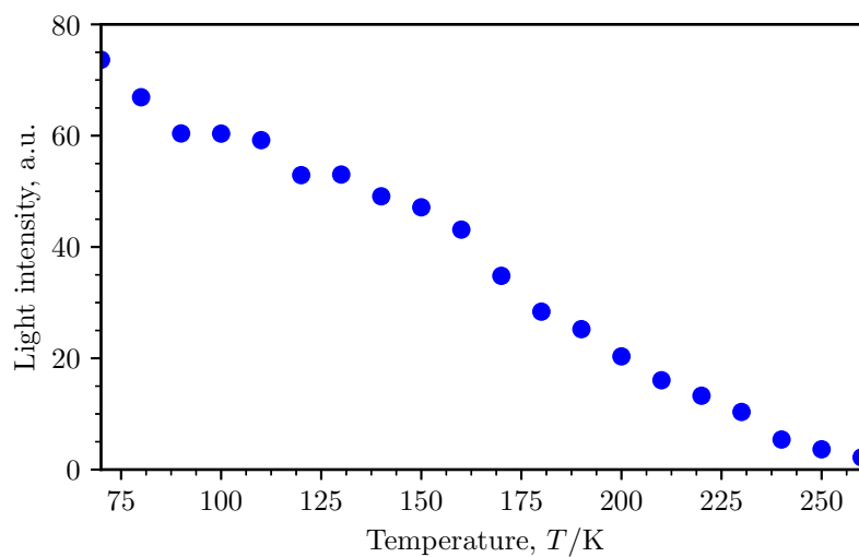
Figure 3.9.: Light intensity (in arbitrary units) of EuTFC embedded in PMMA, baked at 175 °C for 30 min. The range of 4 K to 260 K was investigated in steps of 10 K [104]. Here only the range between 70 K and 260 K is shown, which is interesting for HTS coated conductors.
