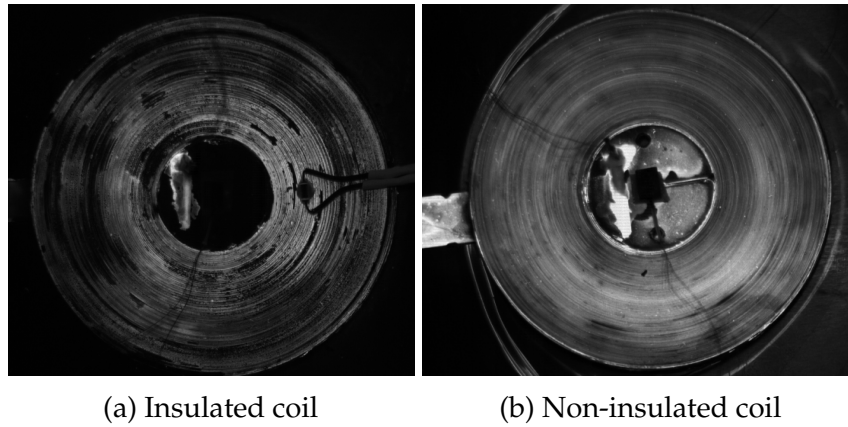
Figure 5.13.: Raw fluorescent image of (a) the insulated coil and (b) the NI coil. The image of the insulated coil already shows a retrofit resistor used as a heater.
