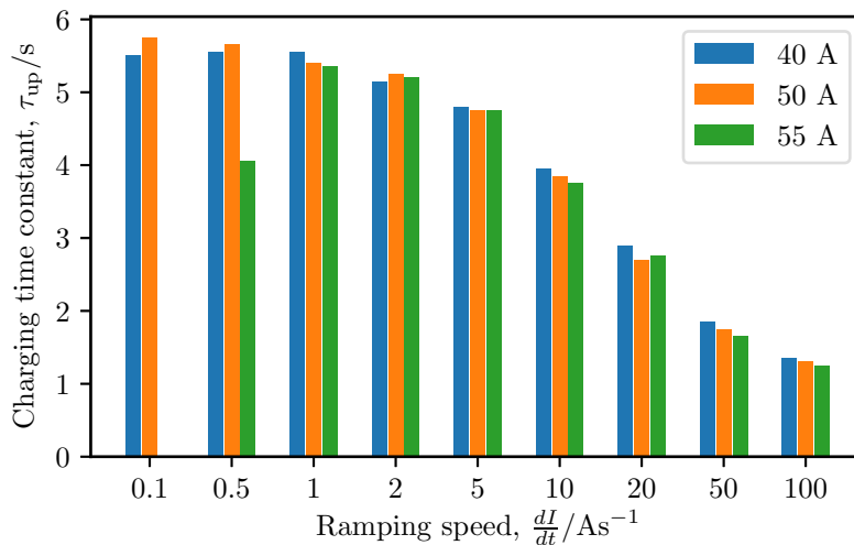
Figure 5.24.: Charging time constant \tau_{\text{up}} of the NI coil as a function of ramping rates between 0.1 \text{ A s}^{-1} to 100 \text{ A s}^{-1} . Data for the 0.1 \text{ A s}^{-1} ramping rate to 55 A is missing.
