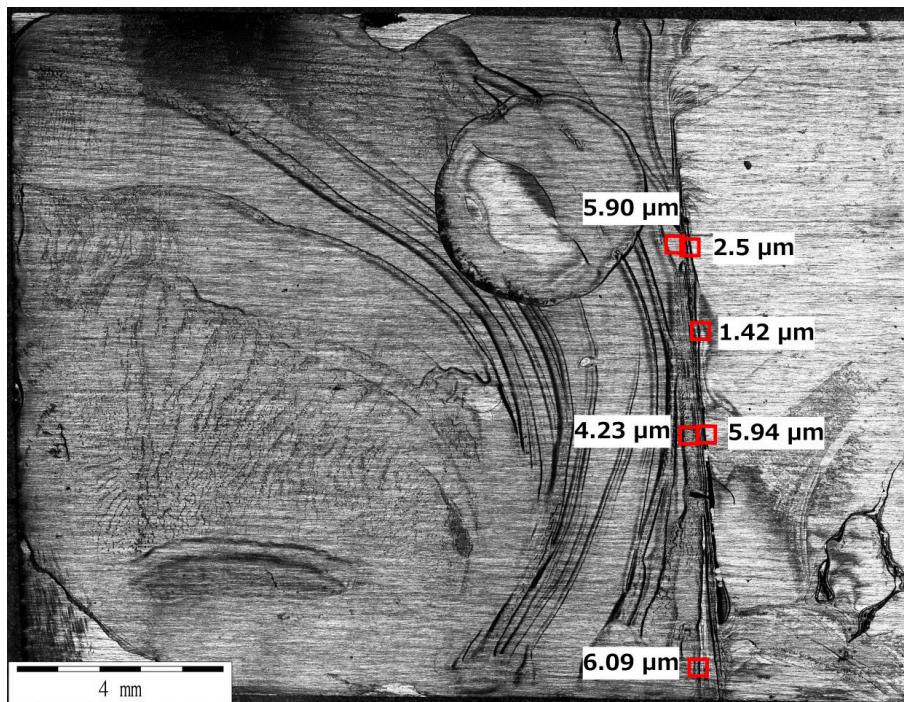
Figure 3.7.: Microscopy image of a steel tape's surface coated until half-way (left) with EuTTA. The red rectangles show areas where atomic force microscopy was used to approximate changes in thickness [103].
