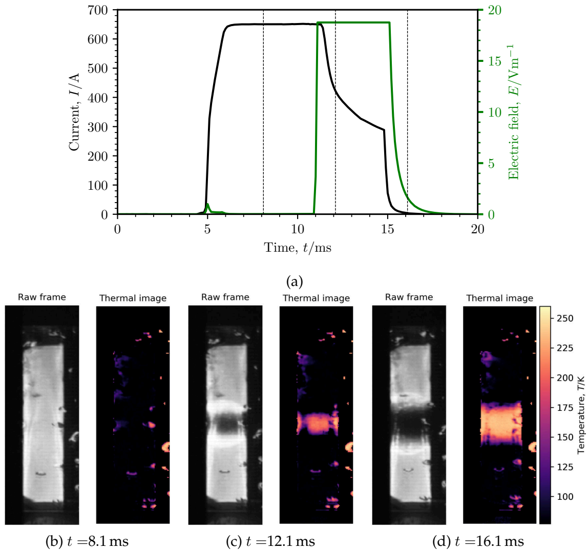
Figure 4.15.: Sample 8 pulsed with a 650 A, 12 ms long pulse. (a) shows the applied current pulse and the recorded electric field across the tape. (b)-(d) show raw and thermal images corresponding to times indicated by the black vertical lines in (a).
