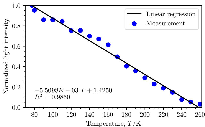
Figure 3.10.: Light intensity of EuTFC embedded in PMMA, heat treated at 175 °C for 30 min and normalized around 77 K. The R^2 value shows a satisfactory fit to a linear approximation.
