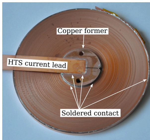
Figure 5.7.: The back-side of the coil showing the 12 mm-wide HTS current lead as well as the coil innermost windings soldered to the coil former.
