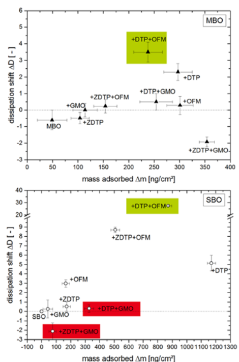
Figure 1 Dissipation and adsorbed masses for two base oils. The green boxes indicate a synergistic effect in terms of wear; the red box indicates an antagonistic effect. The error bars are the standard deviation for three measurements
