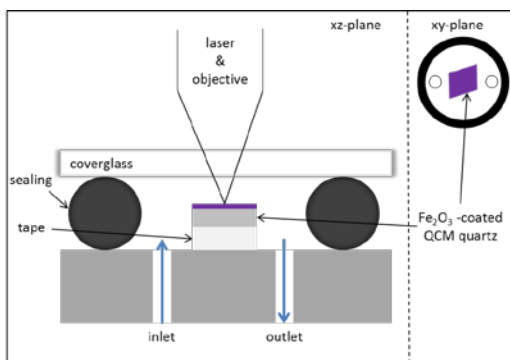
Figure 2 Schematic of the combined QCM-D and CLSM setup.
