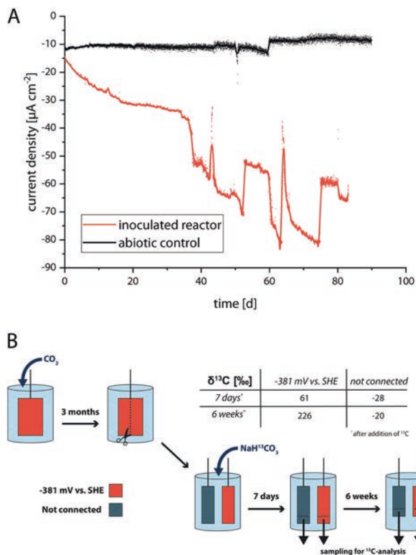
Fig. 1 Chronoamperometric data of the initial cathodic enrichment. a Current density of the initial enrichment reactor (red) and a sterile control (black) over time. Cathodes of both reactors were poised to -381 \text{ mV vs. SHE} . The observed current density fluctuations of the inoculated system correlate with variations in the gas flow ( \text{N}_2/\text{CO}_2 , 80:20, v/v) through the reactor and the compensation of media evaporation by the addition of sterile \text{ddH}_2\text{O} . b Experimental timeline of the ^{13}\text{C} incorporation experiment. The table contains the measured \delta^{13}\text{C} isotopic signatures in parts per thousand [‰]. An integration of the ^{13}\text{C} labeled carbonate is characterized by a positive \delta^{13}\text{C} value.
