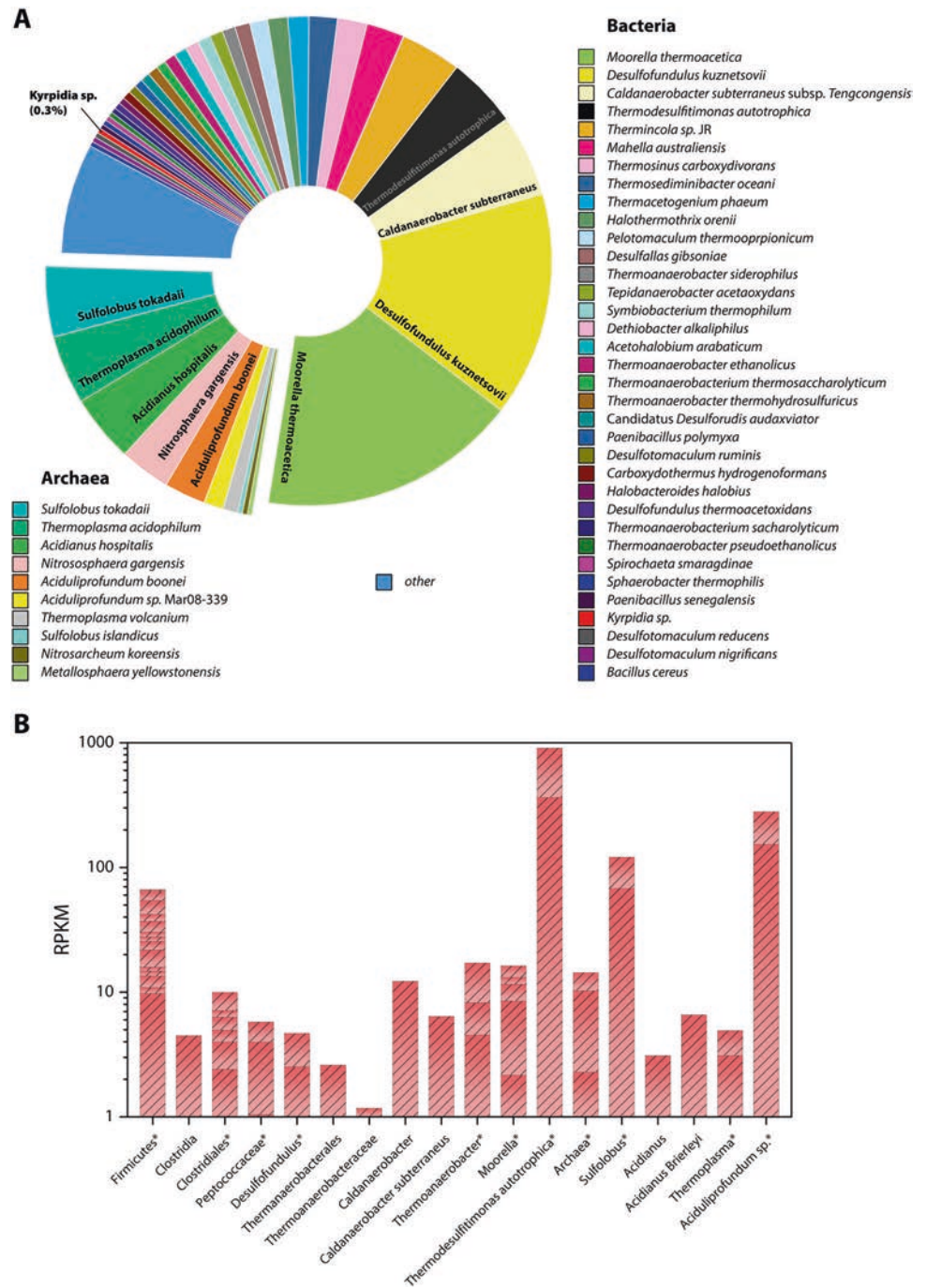
Fig. 2 Metagenome-based phylogeny. a Taxonomic distribution, corresponding to annotated proteins in the metagenome (Only taxa with an abundance >0.2% are depicted; other: unassigned genes and underrepresented taxa with an abundance ≤0.2%; displaced wedges represent archaea). b Taxonomic distribution based on the conducted MetaBat analysis. Filtered raw reads of the metagenome were mapped against the 52 phylogenetic bins. Stacked bars of the asterixed taxa consist of several bins with identical taxonomic contribution. The full summary of all bins can be found in Supplementary Table 2.
