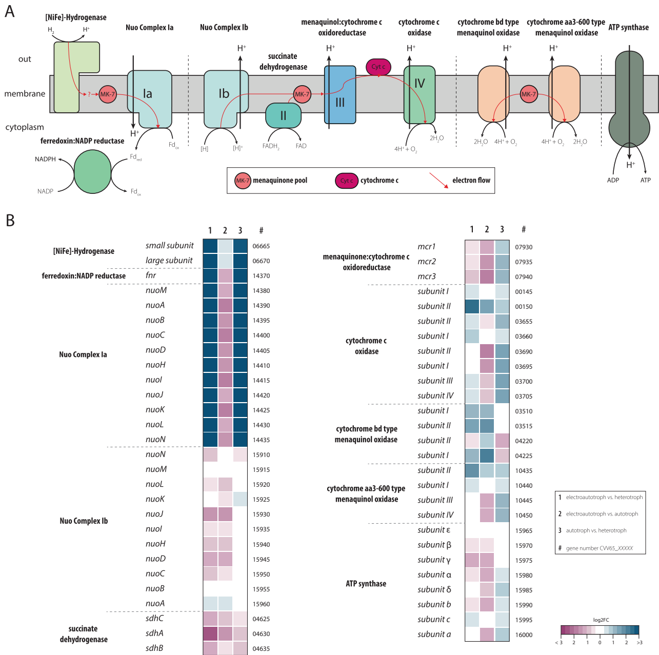
Fig. 6 Scheme and expression of the different modules of energy conservation in K. spormannii . a Model of the branched respiratory chain of K. spormannii based on the transcriptomic analysis.
