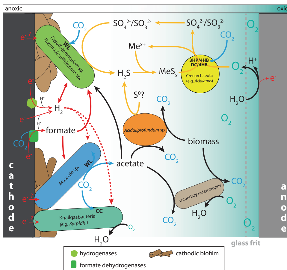
Fig. 3 Scheme of the potential metabolic interactions of the cathodic community, based on the results of the metagenomic analysis. Electrons could be taken up from the cathode either directly or via hydrogen or formate dehydrogenase. These electrons could provide the energy source for Desulfotomaculum species and organisms belonging to the Thermoanaerobacteraceae. The latter would produce acetate as catabolic end product which could be used by a variety of heterotrophic species in the bioelectrochemical system. Hydrogen
