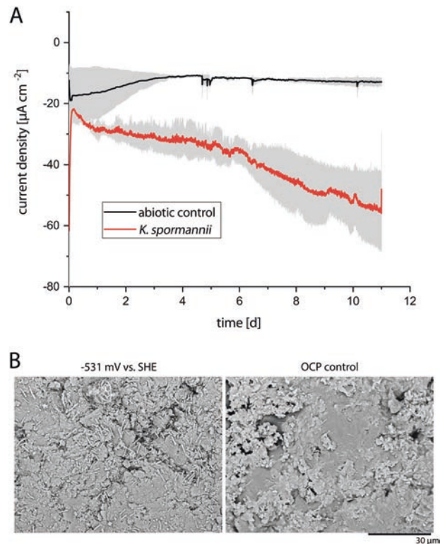
Fig. 4 Electroautotrophic culturing of the isolated K. spormannii . a Chronoamperometric data comparing inoculated electrosynthesis reactors (red) with an abiotic control (black). Cathodes were poised to -531 mV vs. SHE. The sparging gas had an oxygen concentration of 0.5%. Gray error bars represent standard deviation ( n = 3 ). b Representative electron micrographs of the graphite electrodes after 9 days of incubation in an electrosynthesis reactor inoculated with K. spormannii . A cathode that was poised to -531 mV vs. SHE is depicted on the left hand side, whereas the right picture shows an open circuit potential (OCP) control cathode.
