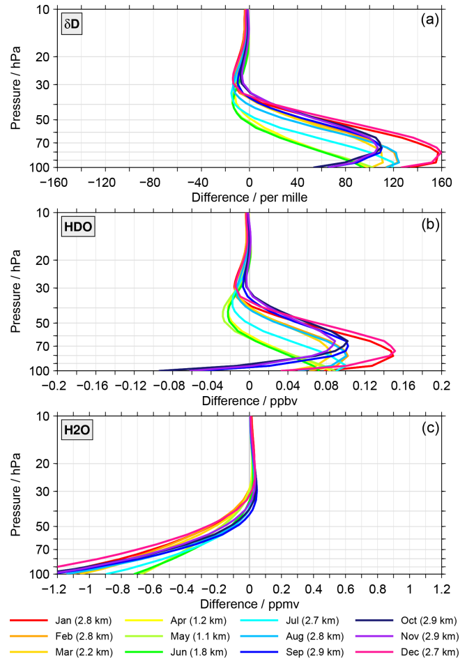
Figure 6. Differences in \delta D (a), HDO (b) and H 2 O (c) between the test and standard retrieval as a function of altitude and colour-coded for the calendar months. The calculation of these monthly mean differences follows Eqs. (A8) and (A11) in the Appendix. In the legend also the change of the start altitude between the two retrievals is indicated for the individual months, derived according to Eq. (A12).
