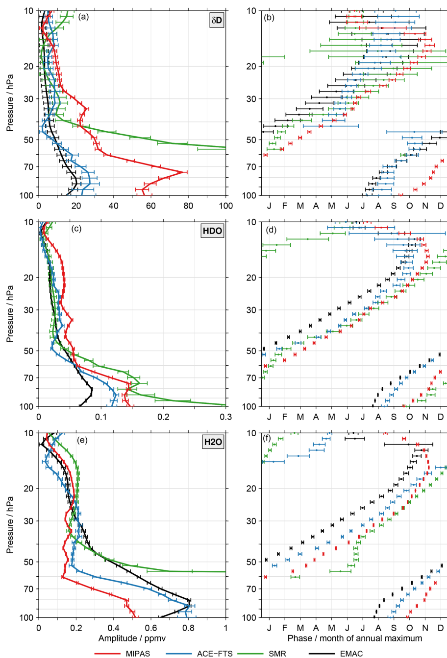
Figure 3. Characteristics of the annual variation for \delta D (a, b), HDO (c, d) and H 2 O (e, f) in the tropical lower stratosphere as derived from the individual data sets. The left panels show the amplitude and in the right panels the phase is given, expressed by the month where the annual maximum occurs. The error bars represent the 2\sigma uncertainty level.
