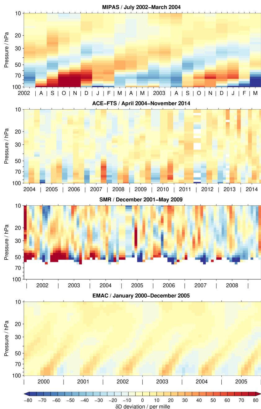
Figure 1. Tropical time series of \delta D deviations from the annual mean covering the altitude range between 100 and 10 hPa. Depending on the data set, a different time period is covered, which is indicated in the individual panel titles. For the EMAC simulation, the time period from 2000 to 2005 is considered arbitrarily. Observational gaps in the data sets are removed for better visibility, in particular for the ACE-FTS data set. A figure without the gap removal is included in the Supplement. White areas indicate that no data are available.
