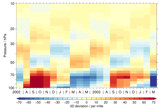
Figure 12. An artificial tape-recorder-like signal resulting from the convolution of EMAC data with the MIPAS averaging kernels of \text{HDO} and \text{H}_2\text{O} . Again, see the text for more details.
