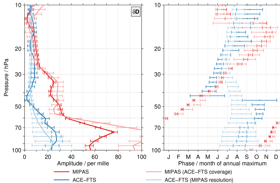
Figure 4. As for Fig. 3 but here focusing on test results for \delta D . Results for a subsampled MIPAS data set that emulates the limited temporal coverage of the ACE-FTS observations in the tropics are shown in light red. The results given in light blue are based on ACE-FTS data whose vertical resolution had been degraded using a Gaussian window with a full width at half maximum of 6 km. The original MIPAS (red) and ACE-FTS (blue) results are shown for comparison.
