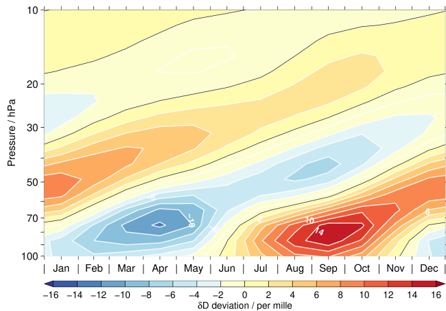
Figure 11. An artificial tape-recorder-like signal in \delta\text{D} due to differences in the vertical resolution of the \text{H}_2\text{O} and \text{HDO} data. The results are based on a simple test using the higher vertically resolved EMAC data for the latitude band between 15^\circ\text{S} and 15^\circ\text{N} . See text for more details.
