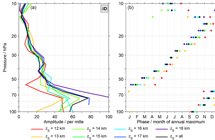
Figure 9. Characteristics of the \delta D annual variation for MIPAS data with specific start altitudes. Panel (a) shows the amplitudes while in panel (b) phase estimates are shown. For the sake of simplicity, no error bars are provided, unlike in Figs. 3 and 4.
