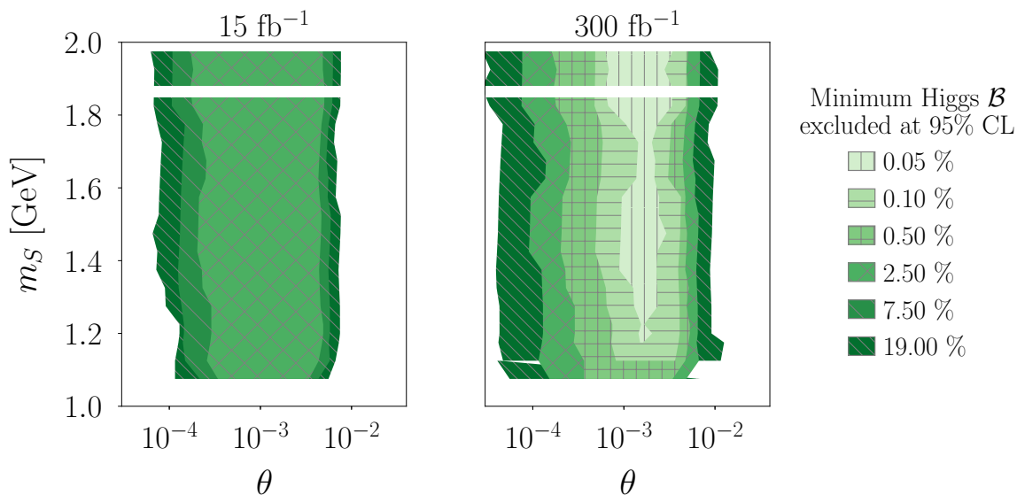
Figure 5. \text{BR}(h \rightarrow SS) bound for the hadrophilic model with \theta = v/M .
