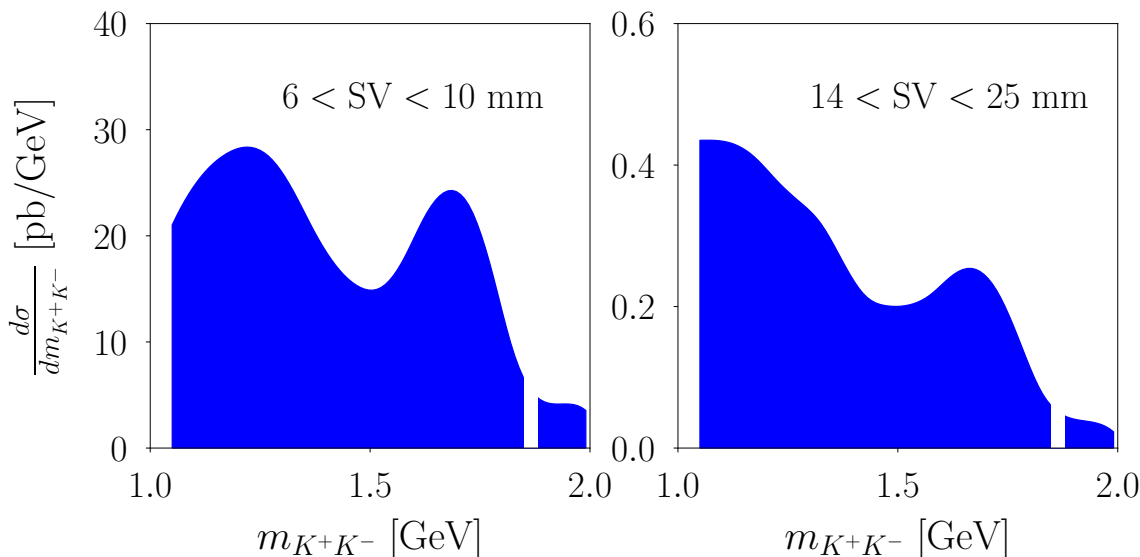
Figure 1. Differential cross section for the b\bar{b} background production after the selection cuts vs. the KK invariant mass. Two of the signal regions, including the selection of a single S scalar with isolation cuts applied are shown. Left (right) correspond to the a_2 ( b_2 ) selections in table 1. We assume the SM Higgs production cross section at \sqrt{s} = 14 TeV. The wiggles are mainly due to the mass vetos applied.
