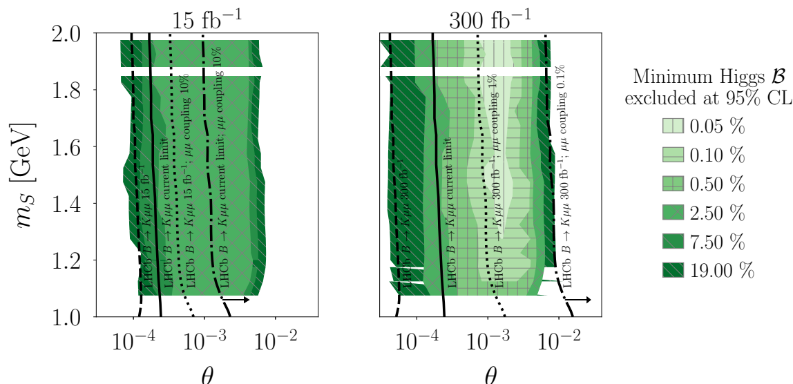
Figure 6. \text{BR}(h \rightarrow SS) bound for the Higgs mixing model. The black solid lines in both plots give the upper bound on \theta from the existing LHCb B^+ \rightarrow K^+ S(\mu^+ \mu^-) search [43]. The black dashed curves show the projected upper bound of the same B -meson search at given luminosities, assuming the search remains background free. In the 15 \text{ fb}^{-1} plot, the dotted and dot-dashed curves give the variation of the existing and future bounds by assuming the S coupling to muons is 10% of \theta m_\mu/v comparing to eq. (4.3). In the 300 \text{ fb}^{-1} plot, the dotted and dot-dashed curves give the variation of the future bounds assuming the S coupling to muons is 1% and 0.1% of \theta m_\mu/v .
