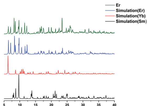
Fig. 6 Comparison of PXRD ErLH 6 with the simulation (Er, Sm, and Yb).
