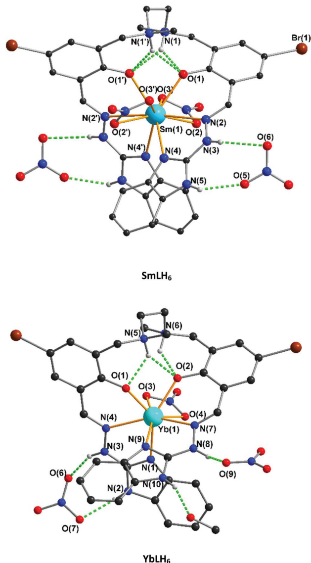
Fig. 3 The structure of SmLH 6 and YbLH 6 . Colour codes for the atoms: light blue (Sm and Yb), blue (N), red (O) black (C) and brown (Br). The hydrogen bonds are highlighted in green dashed line. Solvent molecules (MeCN) in lattice and H atoms are omitted for clarity.
