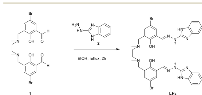
Fig. 2 Preparation of Schiff-base ligand LH 6 .
