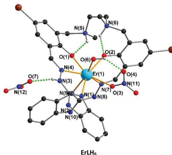
Fig. 5 The structure of ErLH 6 . Colour codes for the atoms: light blue (Er), blue (N), red (O), black (C) and brown (Br). The hydrogen bond is highlighted in green dashed line. Solvent molecules (MeCN) in lattice and H atoms are omitted for clarity.
