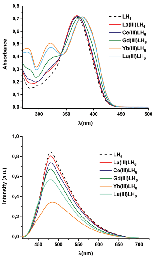
Fig. 7 UV-vis and fluorescence spectra of LH 6 compared with LaLH 6 , CeLH 6 , GdLH 6 , YbLH 6 and LuLH 6 complexes in 50 \mu\text{M} in DMSO ( \lambda_{\text{exc}} = 390 \text{ nm} ).
