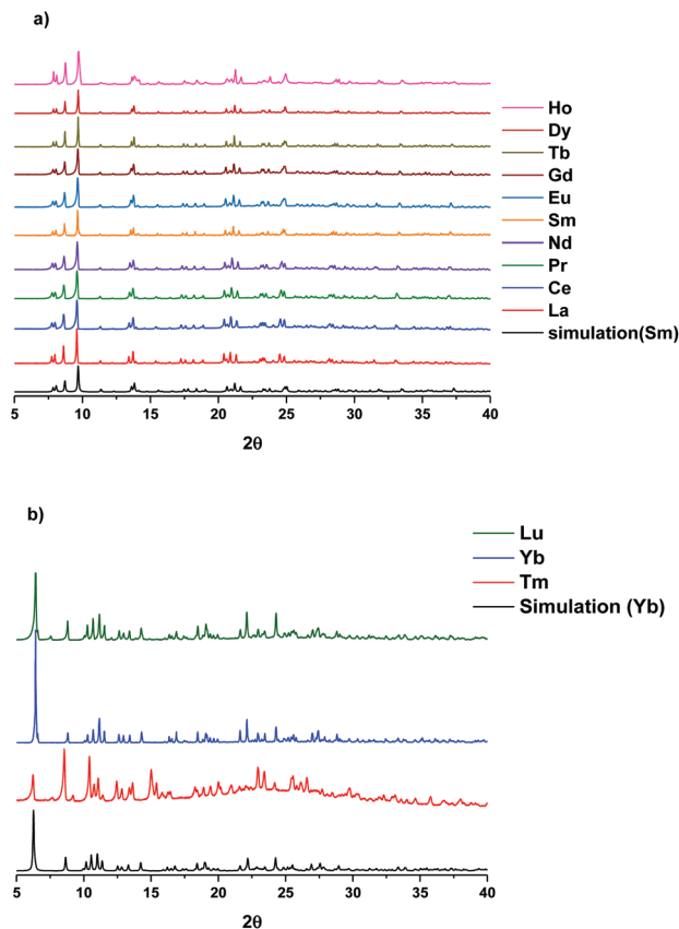
Fig. 4 PXRD of measured Ln(III)LH 6 compare to simulation (a) 10-fold coordination and (b) 8-fold coordination.
