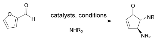
Fig. 1 Transformation of furfural to a trans -4,5-diaminocyclopentenone.
