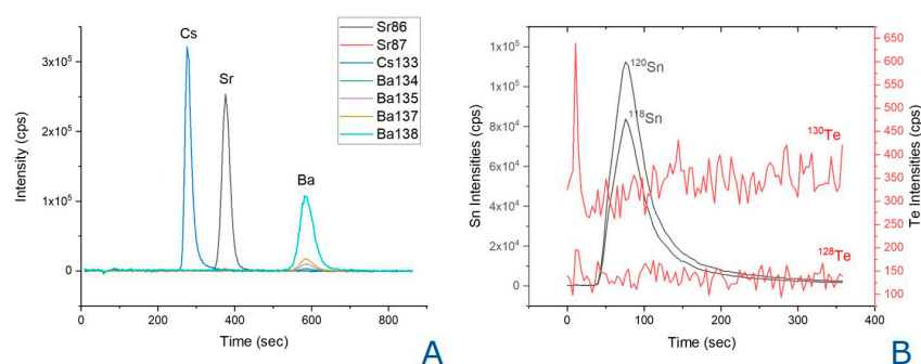
Figure 6. SeaFAST with ICP-DRC-MS time resolved signal of (A) a standard solution of Cs, Sr, and Ba ( 500 \text{ pg g}^{-1} ) on the Ion Pac CS12A column using methanesulfonic acid (MSA) 20 \text{ mmol L}^{-1} as eluent (B) in \text{HNO}_3 1 v/v% using a Nobias chelate-PA1 chelating column using as eluent Acetate 0.5 \text{ mol L}^{-1} pH 6.
