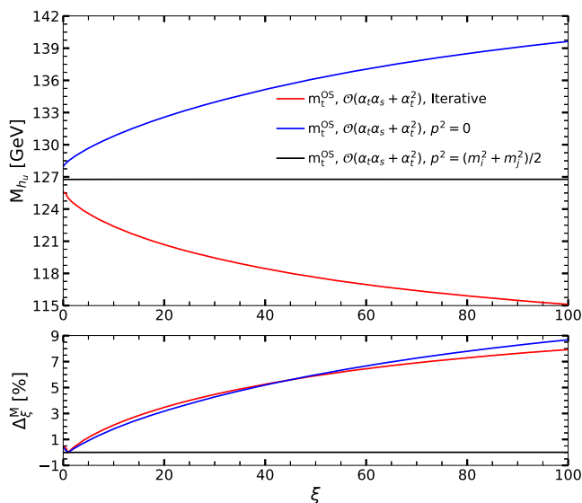
Right: The h_u -like Higgs boson mass of scenario P2 as a function of \xi by applying iterative (red), the R^0 (blue) and the R^{\text{mtree}} -method (black). Lower panels: The corresponding \Delta_{\xi}^M values in percent, as a function of \xi
