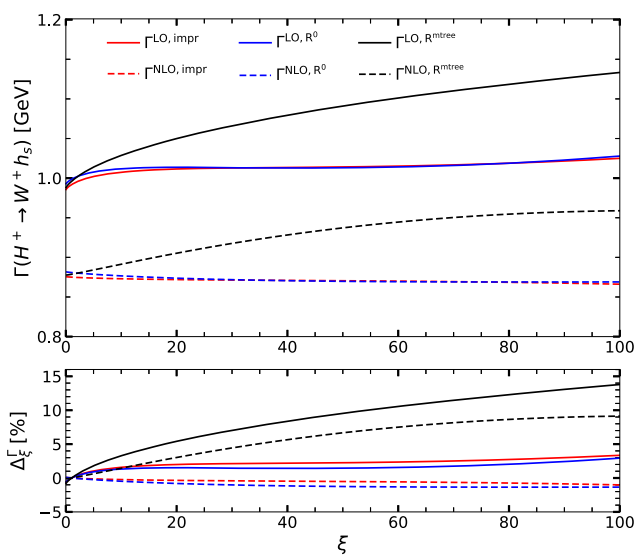
Fig. 15 P2: Decay widths for H^{\pm} \rightarrow W^{\pm} h_u (left upper plot) and H^{\pm} \rightarrow W^{\pm} h_s (right upper plot) as functions of \xi using the iterative (red), the R^0 (blue) and the R^{\text{mtree}} method (black). Lower panels: Corresponding \Delta_{\xi}^{\Gamma} in percent, as function of \xi
