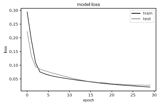
FIGURE 5 Exemplary training history of the reference feedforward network with training hyperparameter set “fit” (number of batches = 1, number of epochs = 30, iterations per epoch = 20). The black line depicts the loss of model training, and the gray line depicts the loss of a random 10% validation split extracted from the training data
