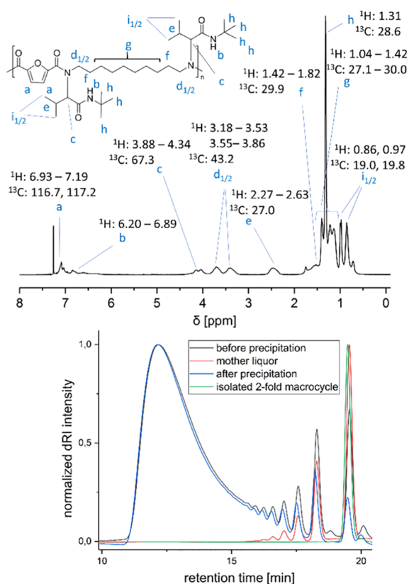
Figure 2. 1 H NMR spectrum (in CDCl 3 ) of the precipitated Ugi polymer (top) and size exclusion chromatography (SEC) trace (bottom) of the polymer before precipitation, after precipitation, the isolated macrocycle, and the mother liquor of the precipitation. The chemical shifts in the 1 H NMR and via heteronuclear single quantum coherence (HSQC) correlated shifts of the 13 C NMR spectrum are given in parts per million (ppm).
