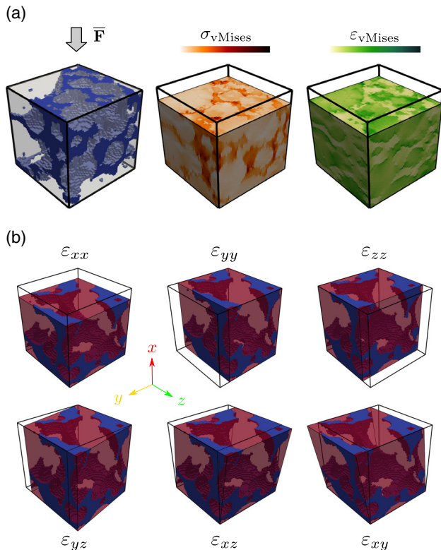
Figure 6. a) 50^3 voxel foam structure under pressure load. Qualitative von Mises stresses and strains resulting from a prescribed compression in x -direction. b) The six independent load cases (pressure in x -, y -, and z -direction and shear in yz -, xz -, and xy -direction) applied to determine the stiffness matrix C of the foam or composite. Here, an MMC of 50 voxel edge length with the \text{Al}_2\text{O}_3 shown in blue and the \text{AlSi10Mg} in transparent red is used as an example.
