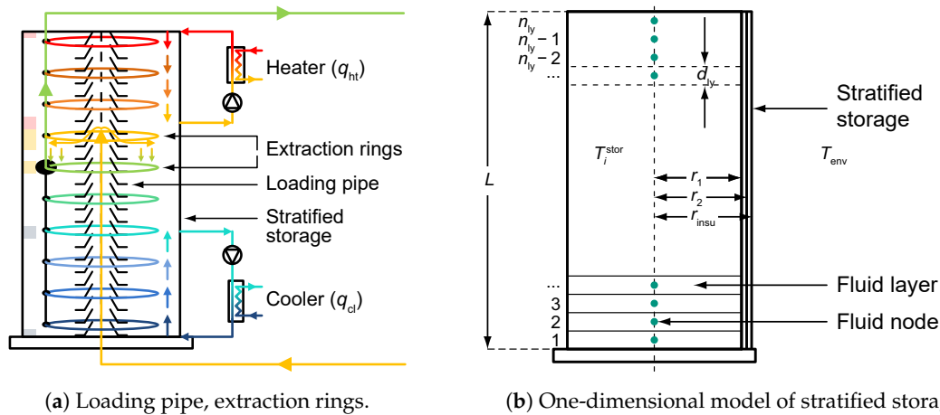
Figure 2. Storage concept with (a) passive loading pipe and rings for extraction, and characteristics of the storage model (b). Colors represent temperatures qualitatively. Convection due to external mass flows is shown on the left (red squares: heater, yellow: adsorber, blue: cooler).
