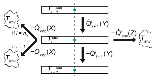
Figure 3. Heat balance of a fluid node in storage. Arrows denote the dominating direction. The forced mass flows through adsorber, heater, and cooler are modeled using (fractional) plug flow. Other convection and the vertical conduction are represented by Q_{i\pm 1}^i(Y) . Losses to the environment are denoted by Q_{\text{env}}^i(Z) (wall) and Q_{\text{cap}}^i(X) (cap, bottom).
