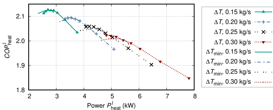
Figure 8. COP plotted over heating power for varied system mass flow ( \dot{m} = 0.15, 0.2, 0.25, 0.3 \text{ kg s}^{-1} ), minimal driving temperature difference at the adsorber ( \Delta T = \{0, 1, 2, 3, 4, 5, 7, 10\} K), and minimal temperature difference across the adsorber for half cycle switching ( \Delta T_{\min} = \{1, 2, 3, 5, 7, 10, 15, 20\} K). The standard values are shown in bold face. Figure adapted from [10].
