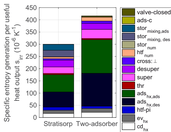
Figure 6. Comparison of the various irreversibilities between the Stratisorp and a two-adsorber system with thermodynamically optimized switching of return flows. The entropy production is normalized for the useful heat released over a cycle Q_{\text{rj}} = Q_{\text{cl}} + Q_{\text{cd}} (neglecting Q_{\text{l}} ). Figure adapted from [10].
