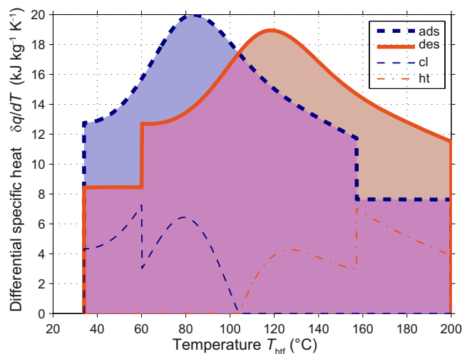
(a) Differential heat for water–zeolite Li-Y.
