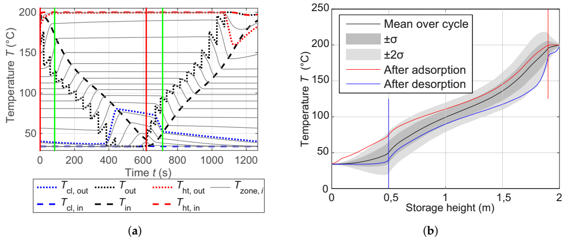
Figure 5. (a) Evolution of the temperature in the storage over a cycle and (b) the temperature profile in the storage after each half cycle along with a statistical evaluation.
