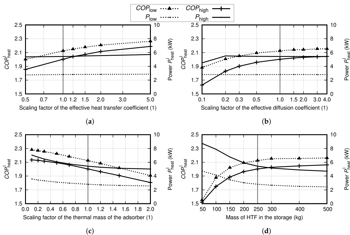
Figure 7. Sensitivity analysis on the COP and heating power of the Stratisorp system on (a) scaling the heat transfer coefficient between the adsorption site and the HTF, (b) scaling the mass transfer coefficient between the adsorption site and the evaporator or condenser, (c) scaling the sensible thermal mass of the adsorber, and (d) varying the mass of fluid in the storage. The subscripts “high” and “low” represent system mass flow rates of 0.3 \text{ kg s}^{-1} and 0.15 \text{ kg s}^{-1} , respectively. Figures adapted from [10].
