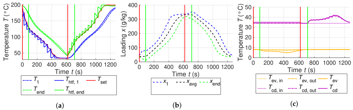
Figure 4. Evolution during the Stratisorp cycle of the (a) temperature and (b) loading in the adsorber, and the (c) temperature in the evaporator and condenser.
