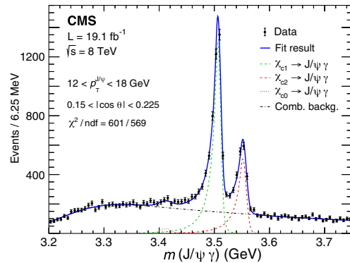
FIG. 1. Example of a fitted J/\psi\gamma invariant mass distribution, for the 0.15 < |\cos \vartheta| < 0.225 bin, in the 12–18 GeV p_T bin. The vertical bars on the points indicate the statistical uncertainties. The lines show the various fit contributions.
