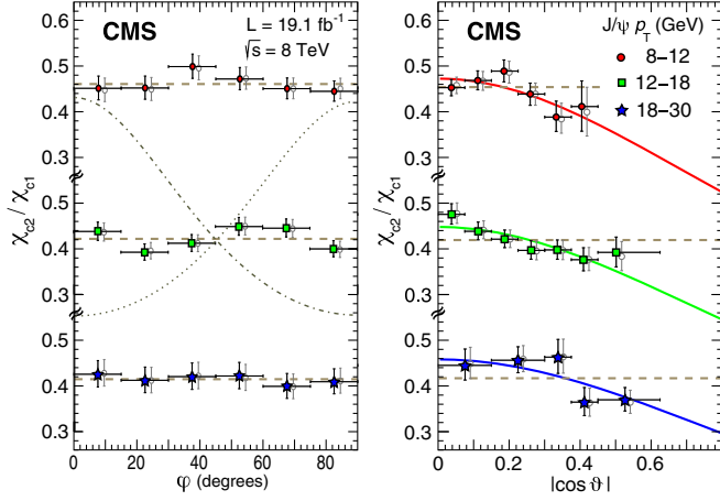
FIG. 2. The \chi_{c2}/\chi_{c1} yield ratio vs \varphi (left) and |\cos \vartheta| (right), for the three J/\psi p_T bins. The gray markers (slightly shifted horizontally) show the values before acceptance and efficiency corrections, scaled vertically for an easier shape comparison. The vertical bars represent the statistical uncertainties and the horizontal bars the bin widths. The solid and dashed curves show, respectively, the NRQCD [43] and unpolarized scenarios. The dotted and dash-dotted curves illustrate maximally different natural polarizations in the Collins-Soper frame, leading to large differences in azimuthal anisotropy.
