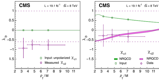
FIG. 4. The \lambda_{\theta}^{\chi_{c1,2}} values (circles) measured when the \lambda_{\theta}^{\chi_{c1,2}} values (squares) are fixed to the unpolarized (left) or the NRQCD (right) scenarios (green curves), as a function of p_T/M of the J/\psi . The purple band on the right is the NRQCD prediction for \lambda_{\theta}^{\chi_{c2}} [43], while in the unpolarized scenario \lambda_{\theta}^{\chi_{c1}} = \lambda_{\theta}^{\chi_{c2}} = 0 . The markers are shown at the average p_T/M values in each bin, the vertical bars represent the total uncertainties, and the horizontal bars the bin widths. The dashed lines indicate the physically allowed range of \lambda_{\theta}^{\chi_{c1,2}} .
