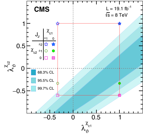
FIG. 3. Two-dimensional \lambda_g^{c2} vs \lambda_g^{c1} contours, at 68.3%, 95.5%, and 99.7% confidence levels (C.L.), measured combining the three J/\psi p_T bins. The physically allowed region (red rectangle) and six pure angular momentum configurations (markers) are also shown. The crossing of the two dashed lines represents the unpolarized case.
