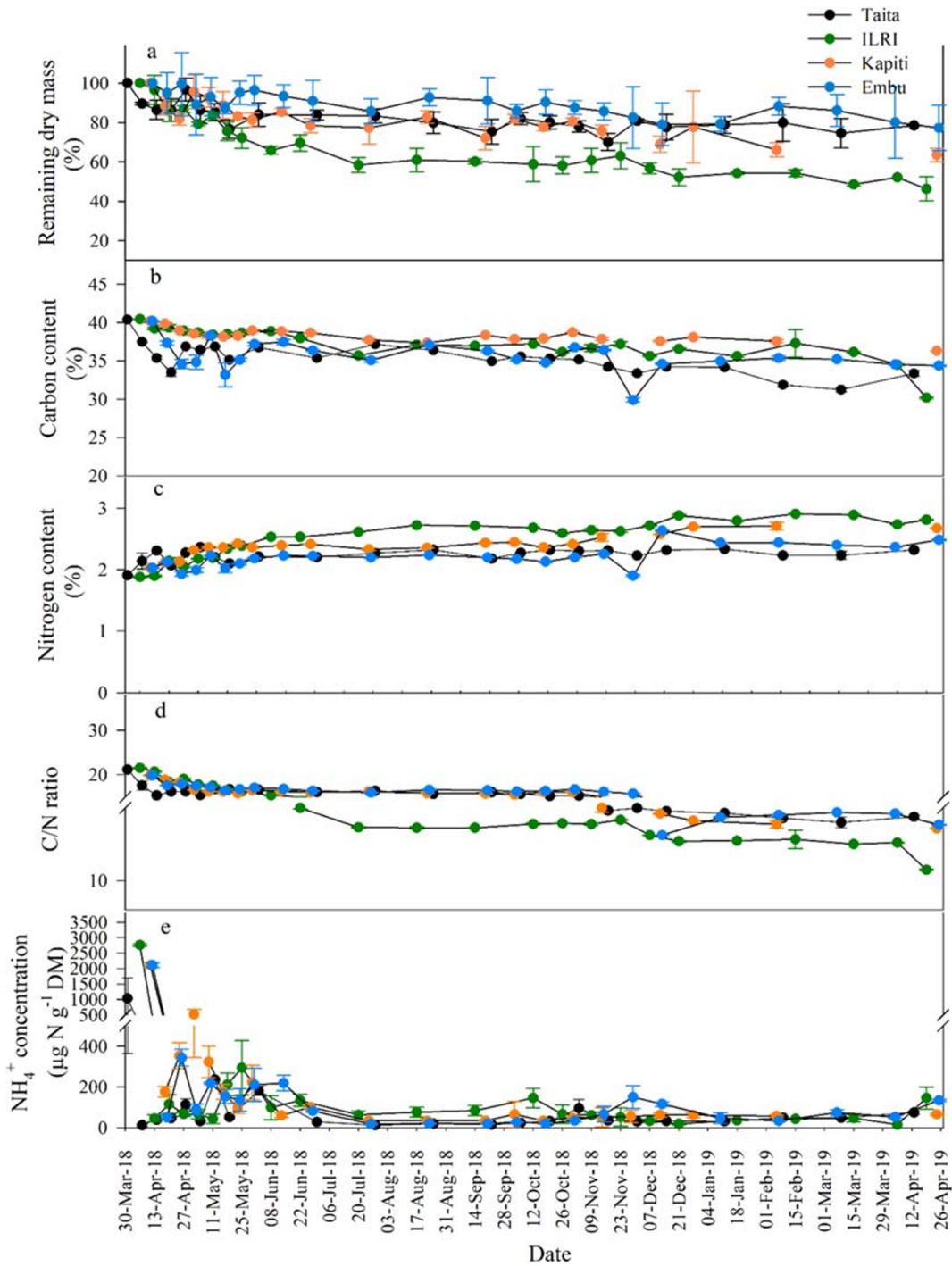
Fig. 7 Dynamics of goat manure remaining as dry mass (a), carbon concentration (b), nitrogen concentration (c), C/N ratio (d) and NH 4 + concentration (e) after litter bags application at Taita,
