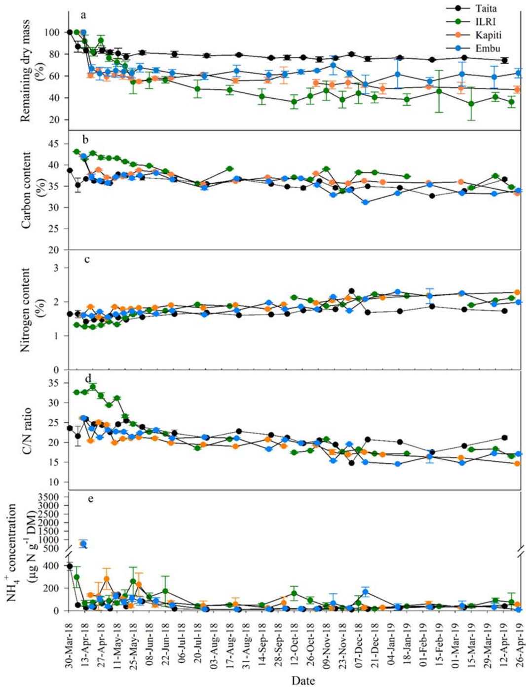
Fig. 5 Dynamics of cattle manure remaining as dry mass (a), carbon concentration (b), nitrogen concentration (c), C/N ratio (d) and NH 4 + concentration (e) after litter bags application at Taita,
