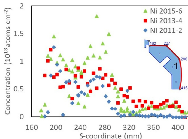
Fig. 1. Nickel concentrations across Tile 1 exposed for each of ILW1, ILW2 and ILW3. The total Ni concentration with respect to Be increased between operating period: 1.4% (ILW1), 1.8% (ILW2) and 2.4% (ILW3). Inset: cross-section of Tile 1 showing the s-coordinates along its surface.
