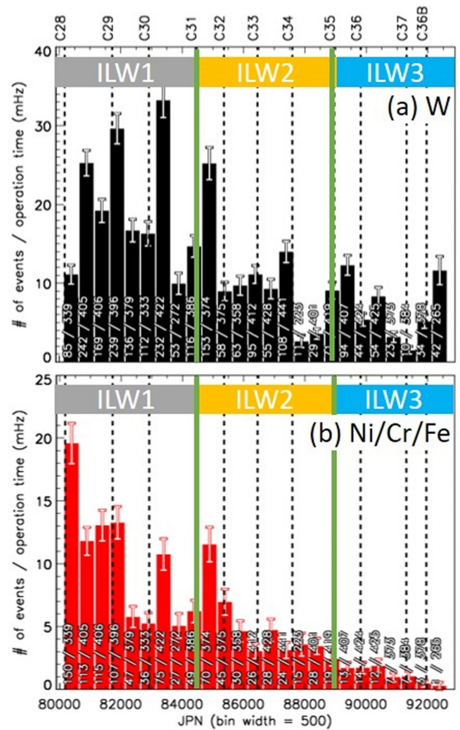
Fig. 6. Transient impurity events for ILW1, ILW2 and ILW3 for (a) tungsten and (b) nickel, chromium iron particles. For each bar the number of TIEs for the given element(s) and total number of TIEs per 500 pulse bin width are shown.
