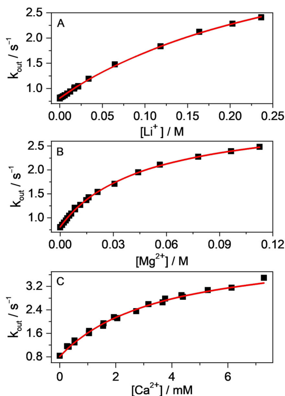
Figure 2. Effect of A) LiCl, B) MgSO 4 and C) CaCl 2 concentrations on the apparent rate constant of B + release from CB7. Lines represent the fitted function.
