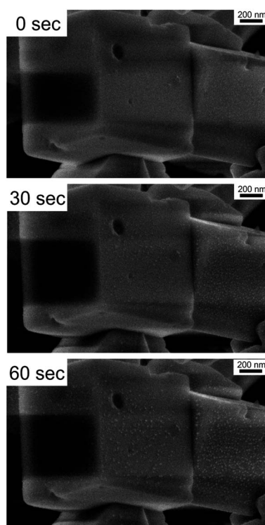
Fig. 4 Evolution of Ag(0) -related spots, up to 10 \pm 4 nm in diameter, due to electron-beam-driven reduction on the surface of \beta-Ag_2MoO_4 cubes after 60 seconds.
