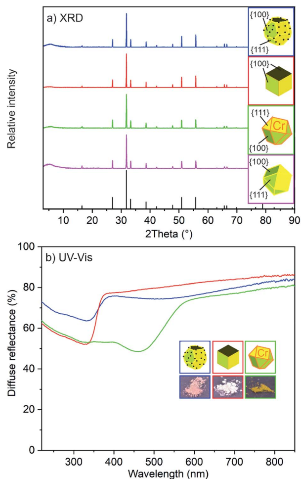
Fig. 5 Crystallinity and optical absorption of the as-prepared \beta-Ag_2MoO_4 microcrystals: (a) XRD (with bulk \beta-Ag_2MoO_4 , ICSD no. 00-070-1497 as a reference) and (b) UV-Vis spectra of truncated Ag_2MoO_4@Ag octahedra (made in DEG; blue); plasmon-resonance absorption indicated by blue star, Ag_2MoO_4 cubes (made in DMSO; red), Ag_2MoO_4 cuboctahedra (made in DMSO; violet), Ag_2(Mo_{0.95}Cr_{0.05})O_4 cuboctahedra (made in DMSO; green) with photos of the respective powder samples.
