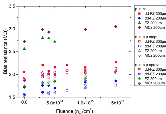
Figure 25. Bias resistance as a function of fluence. The uncertainty in the measured bias resistance is about 1%.
