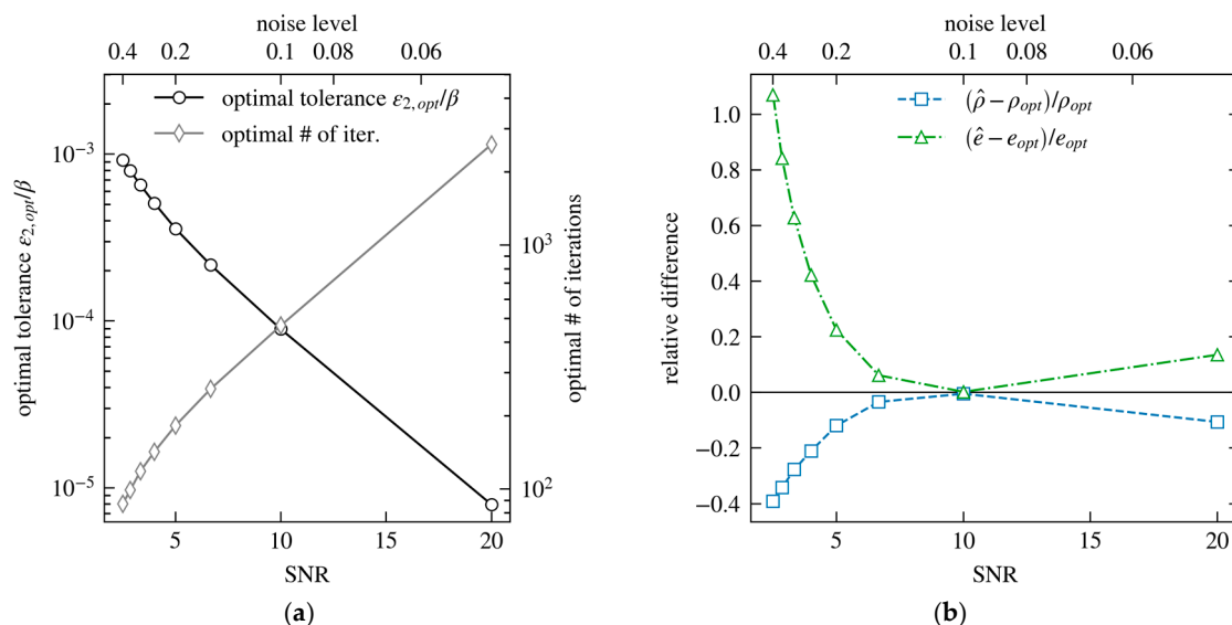
Figure 6. (a) Variation of tolerance \epsilon_2/\beta and number of iterations of the ART algorithm at the point of minimum reconstruction error e_{opt} (compare Figure 5b) as a function of noise level or signal-to-noise ratio (SNR). (b) Relative change between the optimum error e_{opt} or optimum correlation coefficient \rho_{opt} and their values ( \hat{e} and \hat{\rho} ) for a fixed termination criterion of \epsilon_2/\beta = 10^{-4} .
