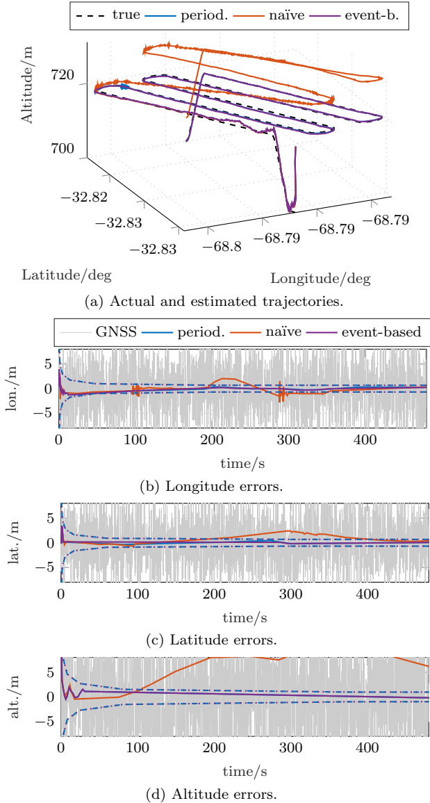
Fig. 2. INS/GNSS navigation example with ADIS16405 IMU error profile. 3\sigma -bounds for the periodic and event-based case are shown as dashed lines.
