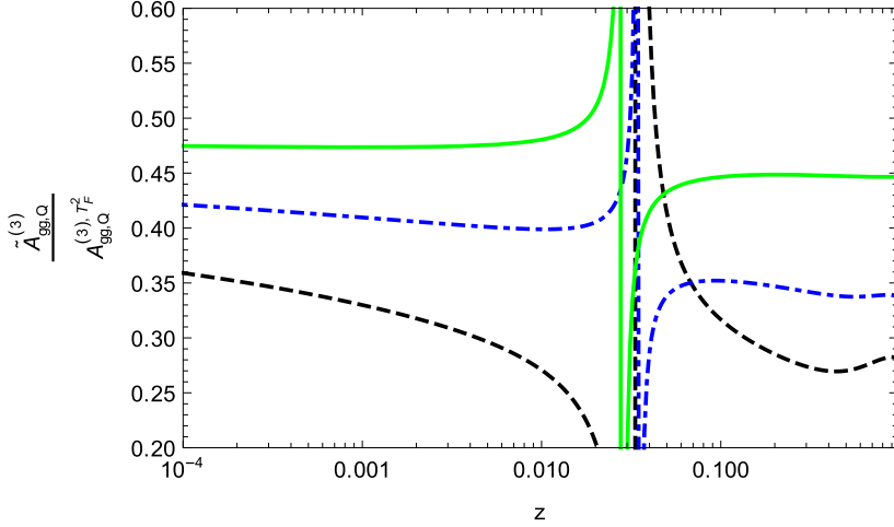
Fig. 2. The ratio of the two mass contribution to the total contribution at O(T_F^2) for the polarized massive OME A_{gg,Q}^{(3)} as a function of the momentum fraction z and the virtuality \mu^2 . Dashed line: \mu^2 = 50 \text{ GeV}^2 ; Dash-dotted line: \mu^2 = 100 \text{ GeV}^2 ; Full line: \mu^2 = 1000 \text{ GeV}^2 . For the values of m_c and m_b we refer to the on-shell heavy quark masses m_c = 1.59 \text{ GeV} and m_b = 4.78 \text{ GeV} [71,72].
