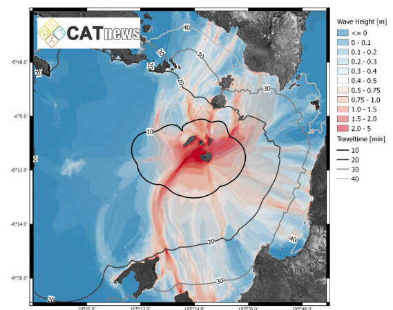
Fig. 1: Combined travel time and modelled wave height map of the 2018 Sunda Strait Tsunami using the model of Schaefer and Wenzel (2017; Source: CATnews).
