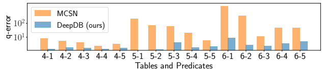
Figure 6: Median q-errors (logarithmic Scale) for different Join Sizes (4,5,6) and Number of Filter Predicates (1-5).
