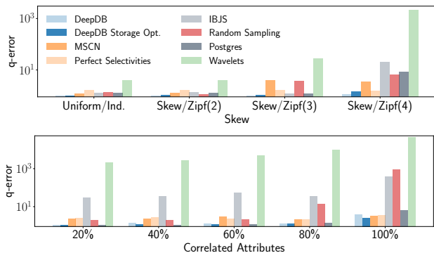
Figure 5: Mean Estimation Errors for Synthetic Data.
