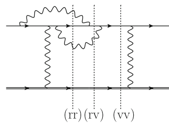
(a) Example for a contribution to the squared matrix element \propto q^6 Q^2
