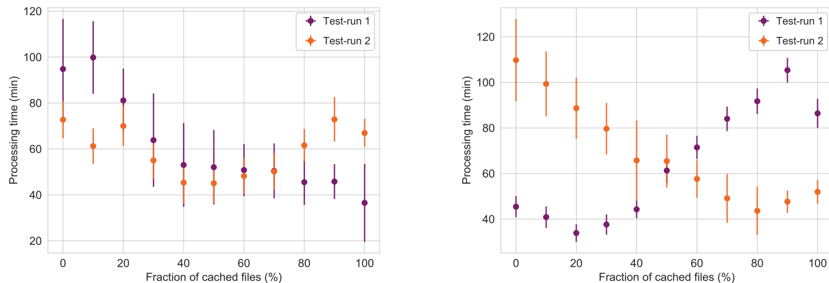
Figure 3. Maximum achievable performance using a cache within the shared NEMO HPC center (left) and the shared OpenTelekom cloud (right). The dots show the mean value of 420 jobs processed in parallel, the error bars represent the variance. [7]
