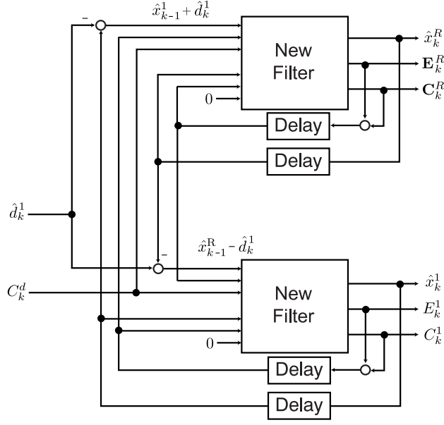
Figure 1. Block diagram of the algorithm for updating the position of wall 1 and the observer position with a measurement \hat{d}_k^1 . Please note, that the observer is assumed motionless for simplicity, which allows to omit the prediction step.
