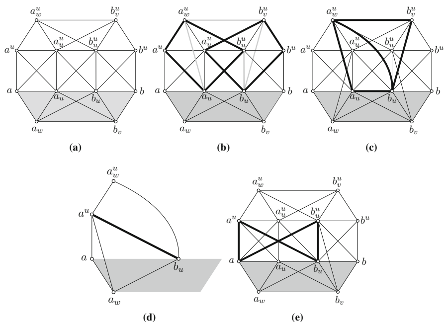
Fig. 12 This illustrates the proof of Lemma 7.9. The last picture on the bottom shows the constructed 4-cycle which does not have a diagonal
