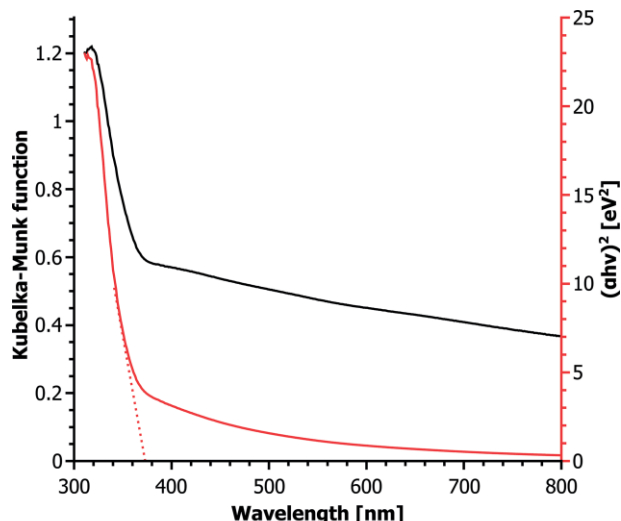
Figure 4. Kubelka-Munk term (black) and Tauc-plot (red) calculated from the observed diffuse reflectivity data of CCS10 showing the broad absorption of CuCo 2 S 4 at higher wavelengths and the absorption edge of TiO 2 at high energies (dotted line).
