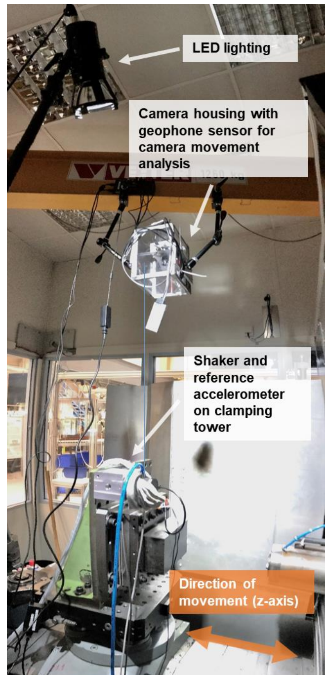
Fig. 1. Setup overview with camera filming moving clamping tower with attached shaker.
