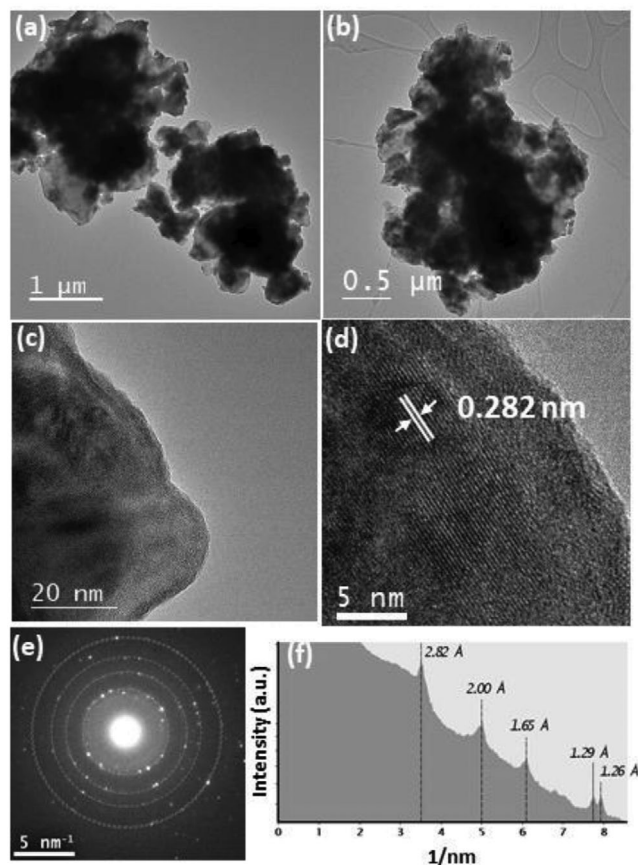
Figure 1. a–c) TEM images of “ \text{Sn}_4\text{P}_3 ”/NHC at different magnifications. d) High-resolution TEM image showing (107) lattice fringes of \text{Sn}_4\text{P}_3 . e) Selected area electron diffraction (SAED) from “ \text{Sn}_4\text{P}_3 ”/NHC. The rings mark the positions of selected strong reflections from \text{Sn}_4\text{P}_3 that are well displayed in an f) integrated average intensity profile calculated from the diffraction ring pattern.
