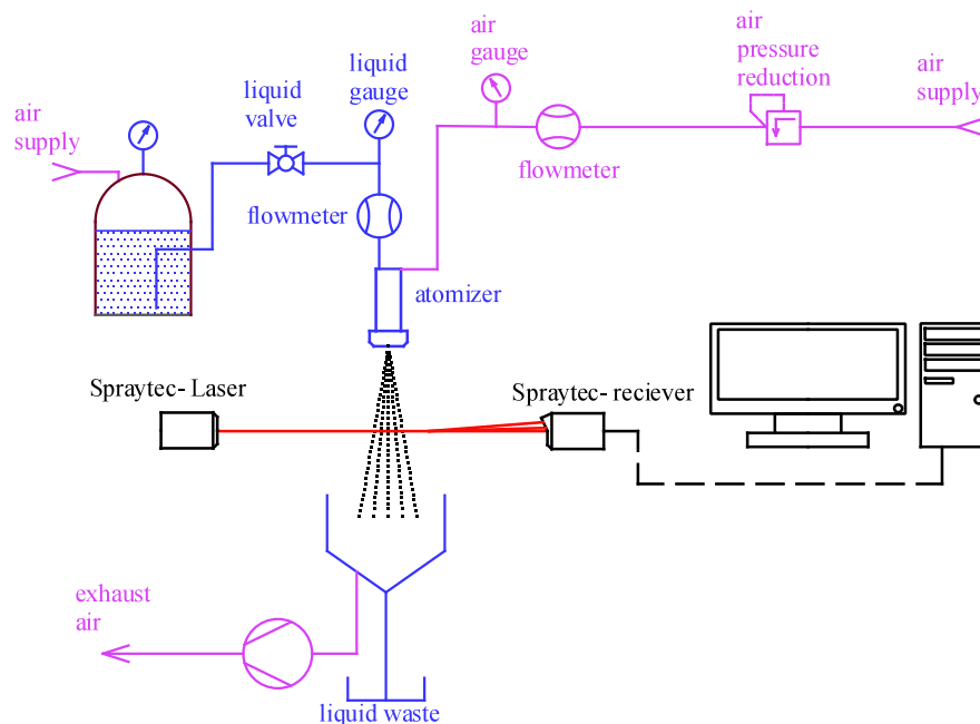
Figure 2. The test rig.
