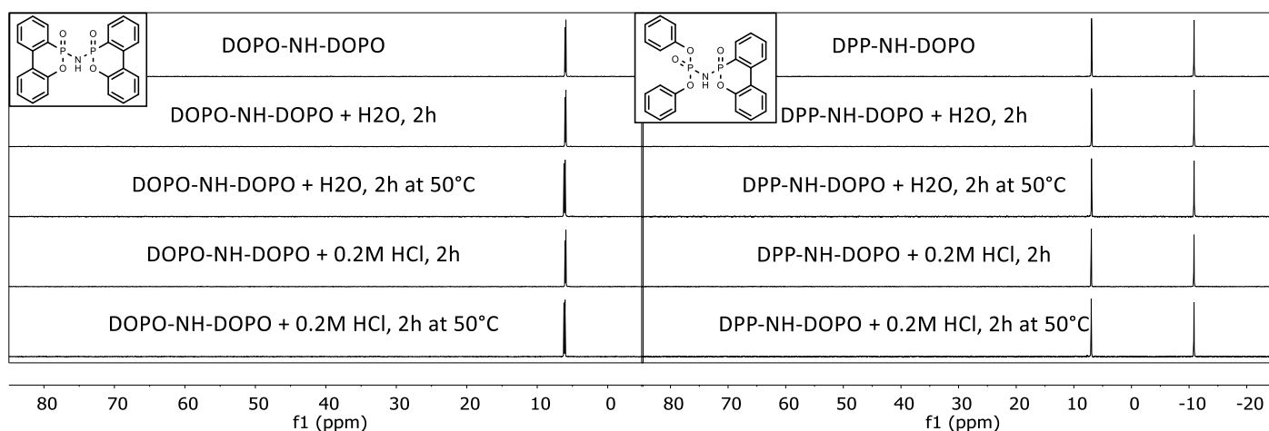
Figure 6. 31 P { 1 H}-NMR spectra of DOPO-NH-DOPO and DPP-NH-DOPO during hydrolysis experiments recorded in a mixture of chloroform-d 3 and Acetonitrile.
