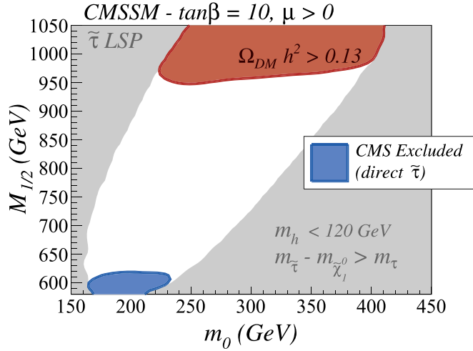
Figure 73. Region of the CMSSM parameter space with long-lived NLSP staus. The light gray regions are excluded by the requirements m_{\tilde{\tau}} \gtrsim m_{\tilde{\chi}_1^0} and 120 \text{ GeV} \leq m_h \leq 130 \text{ GeV} . The top red region is excluded by the upper limit on the neutralino relic density, while the lower blue region is excluded by the CMS constraints on direct production of long-lived staus. For more details see [97].
