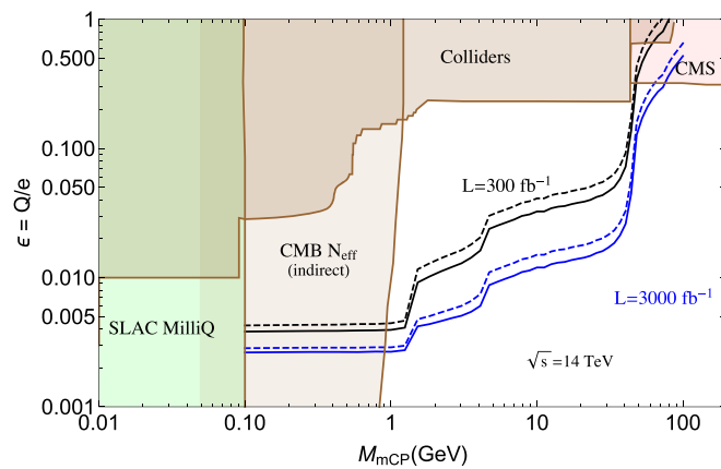
Figure 62. The expected sensitivity of the milliQan experiment for different LHC luminosity scenarios. The black line shows the expected 95% C.L. exclusion (solid) and 3\sigma sensitivity (dashed), assuming 300 \text{ fb}^{-1} of integrated luminosity. In blue is shown the corresponding expectations for 3000 \text{ fb}^{-1} .
