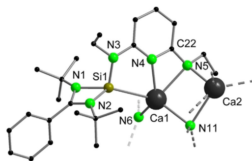
Figure 4. Molecular structure of 4 in the solid state (simplified view). H atoms, the \text{SiMe}_3 groups and non-coordinating solvent molecules are omitted for clarity. Selected bond lengths [ \text{\AA} ] and angles [ ^\circ ]: \text{Ca1}-\text{Si1} 3.0426(15) , \text{Ca1}-\text{N4} 2.314(4) , \text{Ca1}-\text{N5} 2.524(2) ; \text{N4}-\text{Ca1}-\text{N5} 54.55(6) , \text{N4}-\text{C22}-\text{C5} 113.9(2) .
