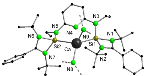
Figure 5. Molecular structure of 5 in the solid state. H atoms and the SiMe_3 groups are omitted for clarity. Selected bond lengths [Å] and angles [°]: Ca–Si1 3.1646(8), Ca–Si2 3.2080(9); Si1–Ca–Si2 92.82(3).
