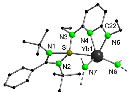
Figure 3. Molecular structure of 3 in the solid state. H atoms and the SiMe 3 groups are omitted for clarity. Selected bond lengths [Å] and angles [°]: Yb1–Si1 3.0426(15), Yb1–N4 2.314(4), Yb1–N5 2.256(4); N4–Yb1–N5 58.93(13), N4–C22–N5 109.9(4).
