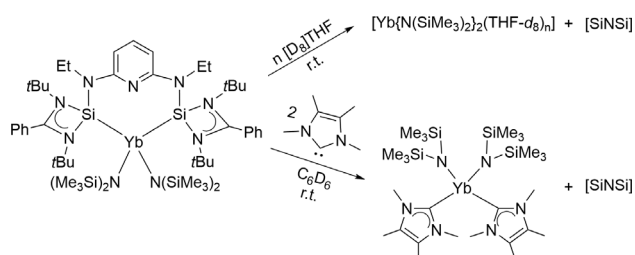
Scheme 2. Reaction of [SiNSi-Yb] ( 2 ) with THF and ITMe.
