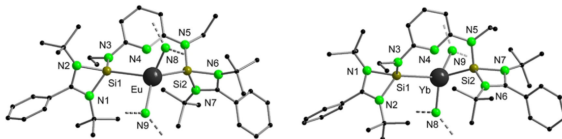
Figure 2. Molecular structures of 1 and 2 in the solid state. H atoms and the SiMe 3 groups are omitted for clarity. Selected bond lengths [Å] and angles [°] in 1: Eu–Si1 3.2810(11), Eu–Si2 3.2875(11); Si1–Eu–Si2 95.25(3); in 2: Yb–Si1 3.1999(11), Yb–Si2 3.1505(11); Si1–Yb–Si2 95.45(3).
