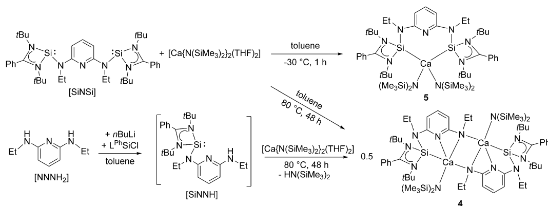
Scheme 4. Different synthetic routes to access complexes 4 and 5 .
