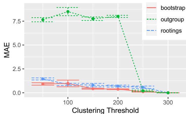
FIGURE 3 MAE (Equation 1) of multiple runs of SCRAPP, using different thresholds down to which placement space clustering (PSC) reduces the maximum per-branch data volume. The MAE is calculated with reference to the case of the threshold being 300, as 300 was the maximum number of QS that were placed per-branch. The underlying query and reference data are from the neotrop data set (Section 3.3, (Mahé et al., 2017))
