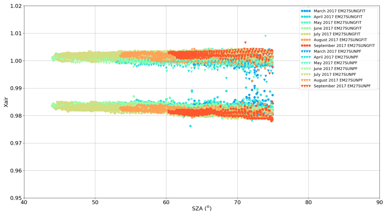
Figure 14. X_{\text{air}} plotted with respect to the measurement solar zenith angle for retrievals performed with EM27/SUN data following COCCON recommendations (EM27SUNPF) and using GFIT (EM27SUNGFIT) for measurements performed at Sodankylä in 2017.
