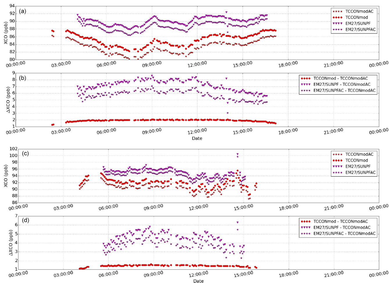
Figure 6. (a) XCO plotted for TCCONmod and EM27/SUN retrievals with the TCCON a priori and with a modified a priori (calculated using in situ, AirCore, and TCCON map files; labelled with AC at the end) for measurements performed on 15 May 2017 at Sodankylä. Panel (b) shows the difference between the two retrievals in absolute units. Panels (c) and (d) show the same plots as mentioned above for measurements performed on 28 August 2017 at Sodankylä.
