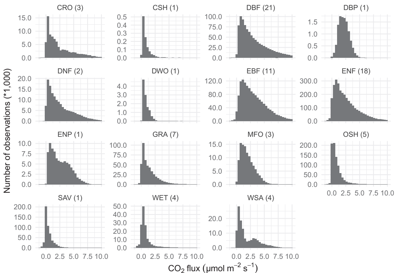
FIGURE 8 Distribution of CO 2 fluxes in COSORE datasets, by IGBP classification (cf. Table 1). For visual clarity this figure excludes fluxes <-1 and >10 \mu\text{mol m}^{-2} \text{s}^{-1} (210,752 observations, 2.6% of the data). Number of datasets (sites) making up data is given in parentheses after IGBP abbreviations in each panel
