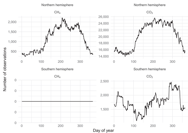
FIGURE 6 Number of observations by day of year, for northern and southern hemisphere and by gas ( CO_2 or CH_4 ), in the current COSORE datasets; the database currently has no CH_4 data from the Southern hemisphere (bottom left)
