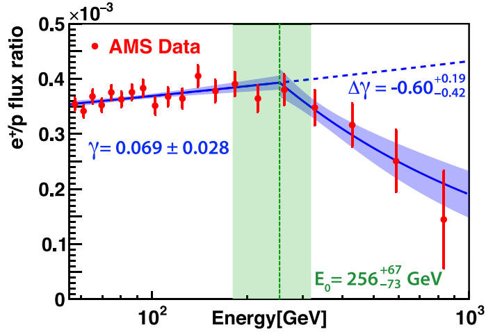
Fig. 67. The ratio of the positron-to-proton fluxes (red data points) together with the fit of Eq. (4) in the energy range [55.58 – 1000]GeV (blue line with 68% C.L. band). As seen, the ratio is rising in the range [55.58 – 256] GeV and decreasing in the range [256 – 1000] GeV. The values of the fit parameters \gamma and \Delta\gamma are shown in the plot together with the transition energy E_0 and its uncertainty (the vertical green dashed line and the green band). The dashed blue line shows extrapolation of the fitted power law function in the range [55.58 – 256] GeV to higher energies.
