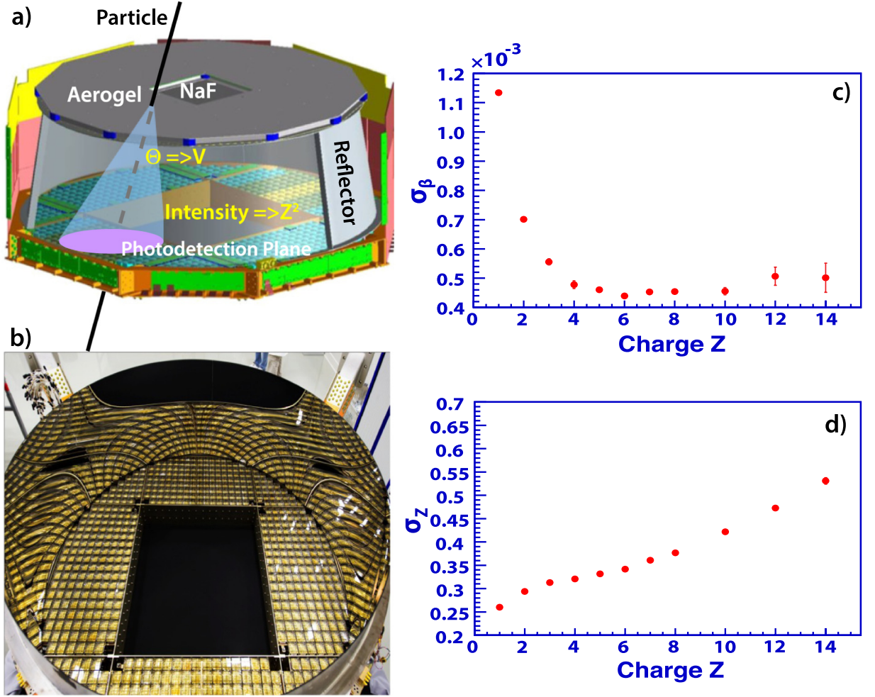
Fig. 24. (a) Schematic of the RICH. (b) The RICH reflector and photo-detection plane. (c) The RICH velocity and (d) charge resolution vs charge Z for the aerogel radiator.
