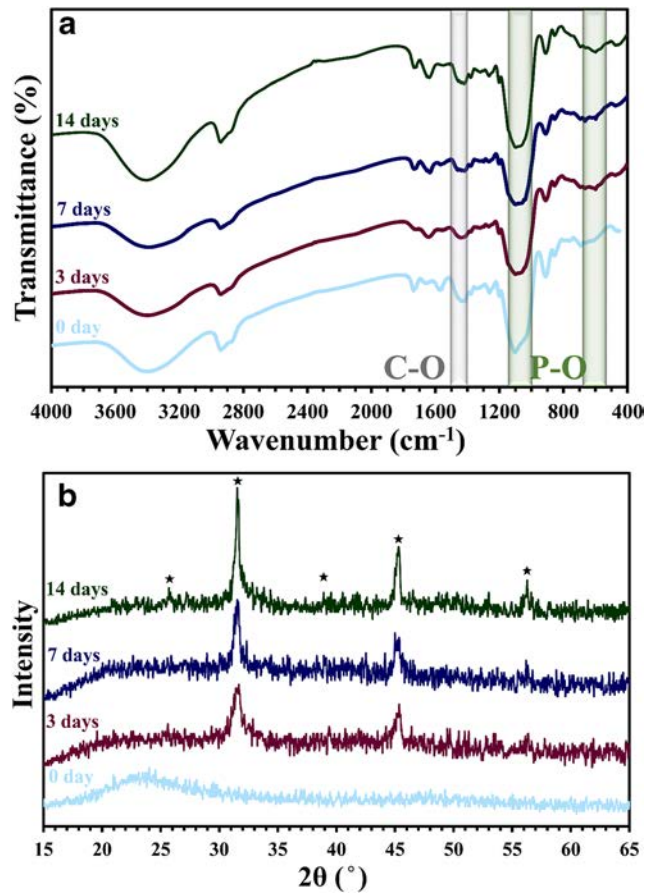
Fig. 8 a FTIR spectra and b X ray diffraction pattern of CP1G scaffolds after different immersion time in the SBF solution
