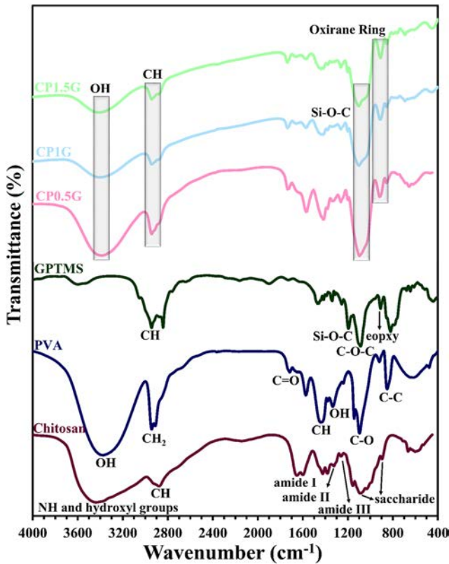
Fig. 3 FTIR spectra of chitosan, PVA, GPTMS, and different scaffolds: CP0.5G, CP1G, and CP1.5G
