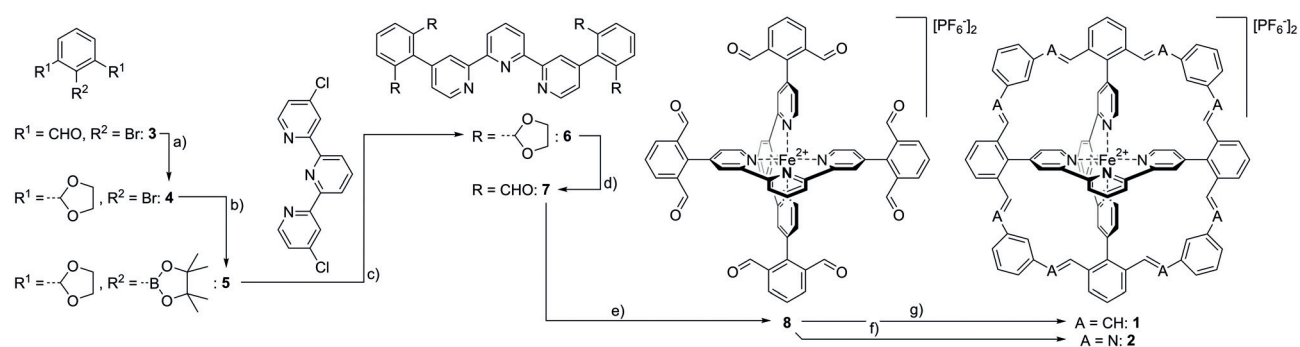
Scheme 1. Synthesis of the Fe(II)tpy 2 cage complexes 2 and 1 . Reagents and conditions: a) Ethylene glycol, p TsOH·H 2 O, toluene, reflux, 12 h, 100%. b) (Bpin) 2 , KOAc, Pd(PPh 3 ) 2 Cl 2 , 1,4-dioxane, 100 °C, 18 h, 87%. c) K 2 CO 3 , Pd(amphos)Cl 2 , toluene/water (5:1), 116 °C, 18 h, 75%. d) PPTS, acetone/water (5:1), microwave (MW), 80 °C, 3 h, 85%. e) 1.) FeCl 2 , DCM/MeOH (1:1), RT, 1 h, 2.) NH 4 PF 6 , water, 12 h, 94%. f) m -phenylenediamine, p TsOH·H 2 O, DCM to DCE, reflux, 10 d, n.d. g) (1,3-phenylenebis(methylene))bis(triphenylphosphonium) dibromide, DBU, DMF, –20 °C, 12 h, 4%.
