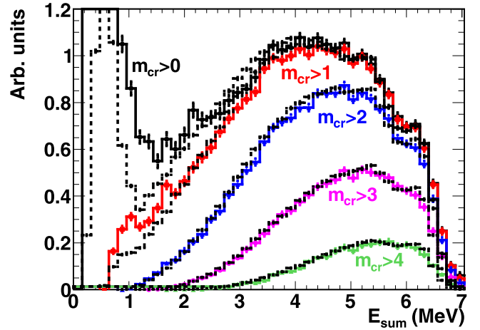
FIG. 11. Experimental (solid lines) and simulated (dotted lines) total deposited energy spectra from ^{235}\text{U}(n, \gamma) cascades for different cuts in m_{cr} , for the geometry with the neutron absorber.
