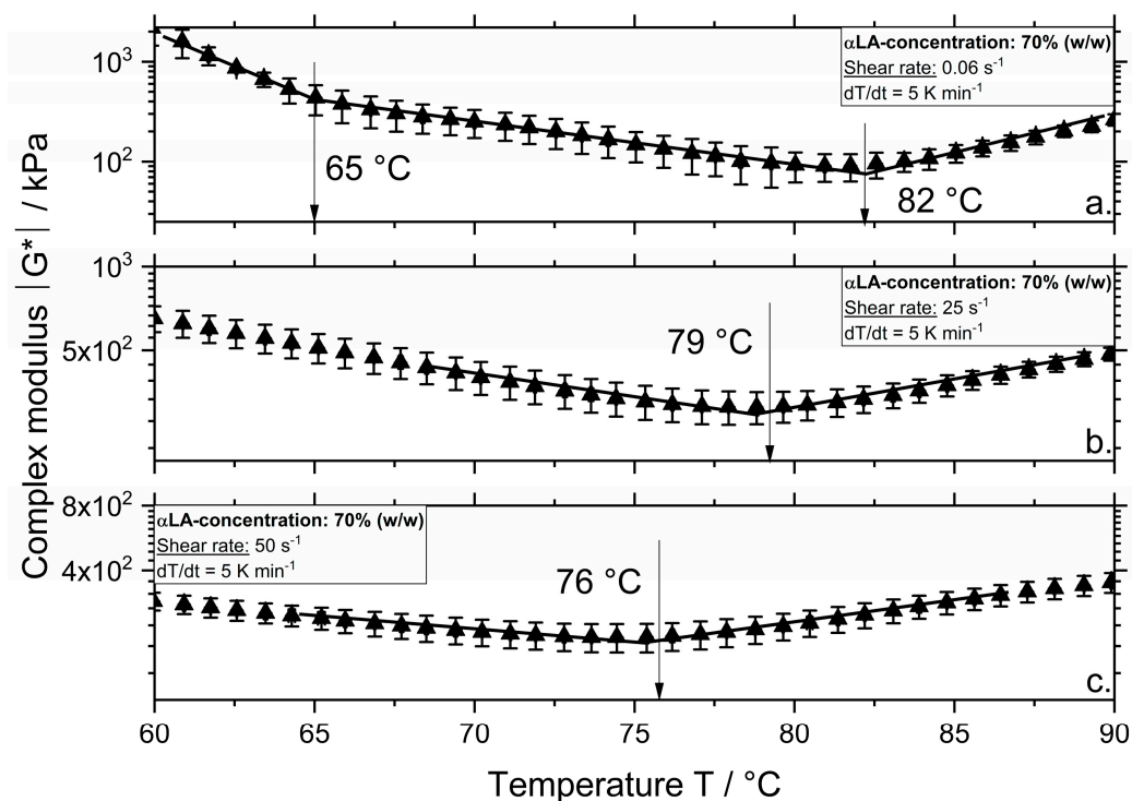
Figure 3. Complex modulus |G^*| as a function of temperature for systems with a \alpha LA concentration of 70% ( w/w ) and a shear rate of 0.06 (a), 25 (b), and 50\text{ s}^{-1} (c). Measurements were performed at a constant heating rate of 5\text{ K min}^{-1} .
