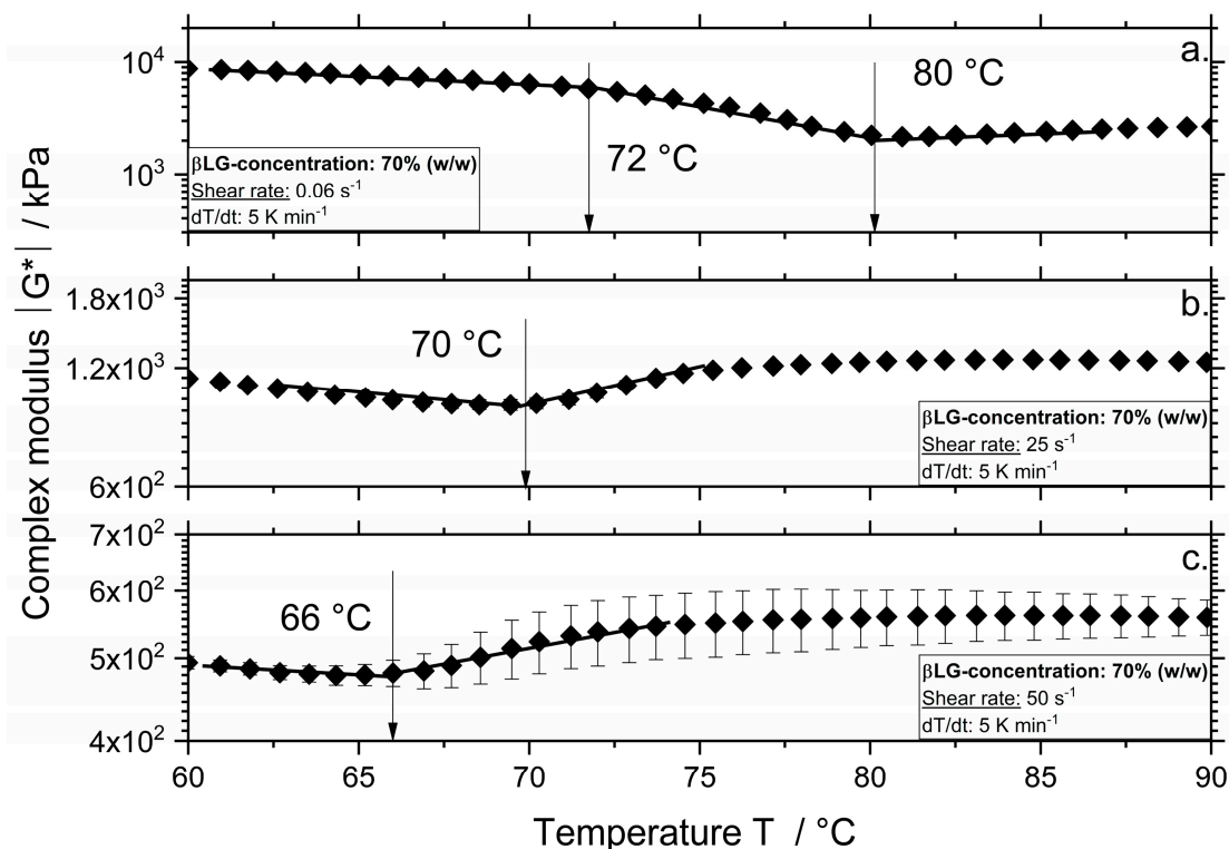
Figure 2. Complex modulus |G^*| as a function of the temperature for systems with a \beta LG concentration of 70% ( w/w ) and a shear rate of 0.06 (a), 25 (b), and 50\text{ s}^{-1} (c). Measurements were performed at a constant heating rate of 5\text{ K min}^{-1} .
